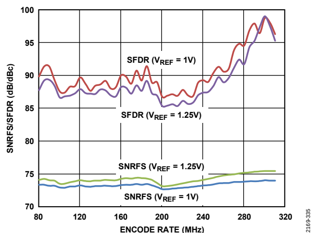
Figure 36. Encode Rate Sweep, f_{IN} = 90.1 MHz at -7 dBFS, V_{REF} = 1.25 V and 1.0 V
