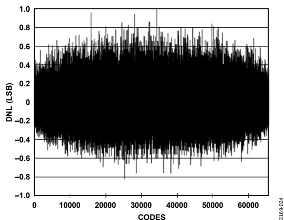
Figure 37. DNL with Dither Off, f_{IN} = 30 MHz
