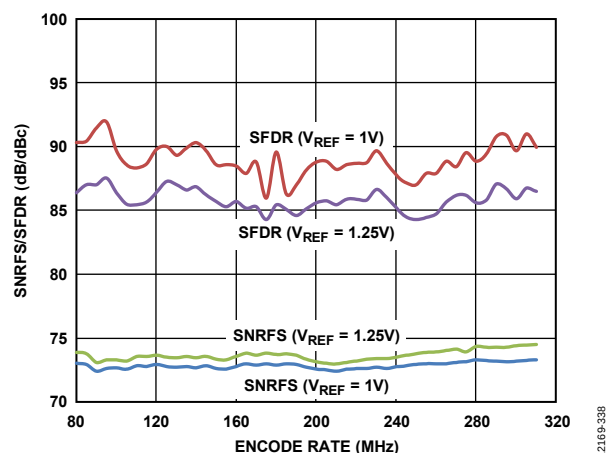
Figure 39. Encode Rate Sweep, f_{IN} = 90.1 MHz at -1 dBFS, V_{REF} = 1.25 V and 1.0 V
