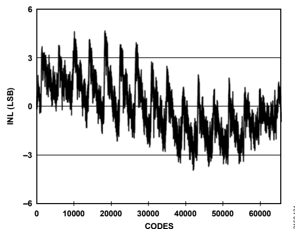
Figure 40. INL with Dither Off, f_{IN} = 30 MHz
