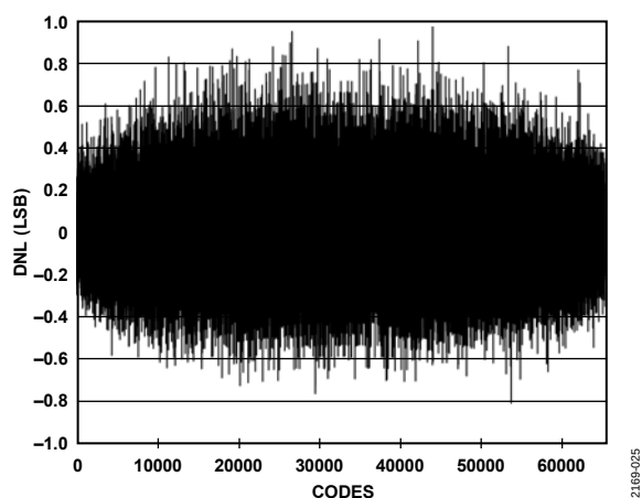
Figure 38. DNL with Dither On, f_{IN} = 30 MHz
