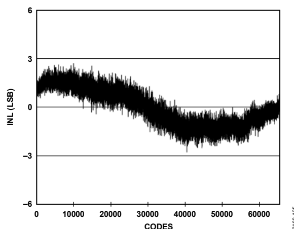
Figure 41. INL with Dither On, f_{IN} = 30 MHz
