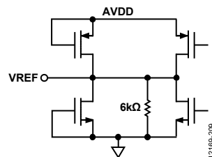
Figure 51. Equivalent VREF Circuit
