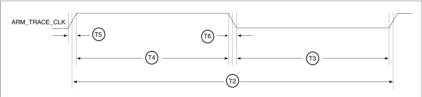
Figure 15. ARM_TRACE_CLK specifications
