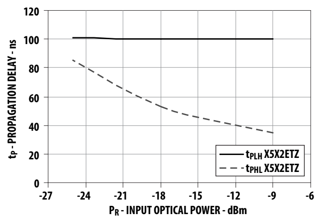
Figure 12: Typical Link Propagation Delay vs. Optical Power
