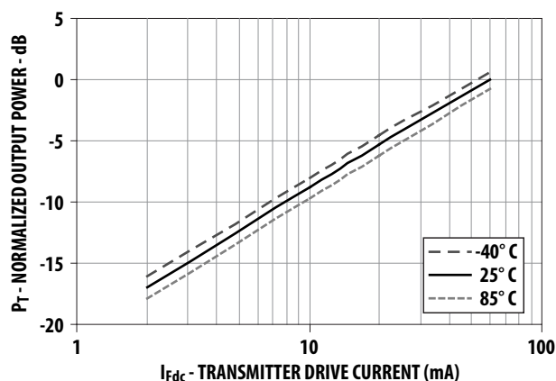
Figure 8: Normalized Typical Output Power vs. Drive Current
