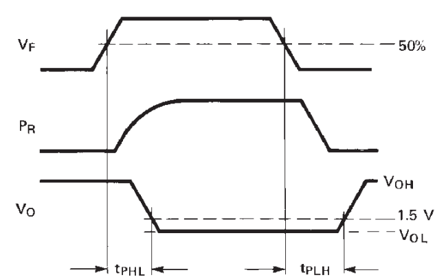
Figure 13: Propagation Delay Test Waveforms
