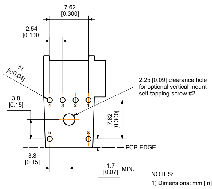
Footprint - TOP VIEW
