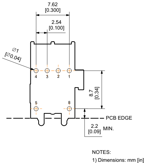
Footprint - TOP VIEW
