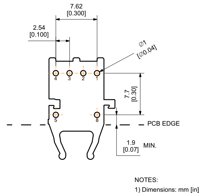
Footprint - TOP VIEW
