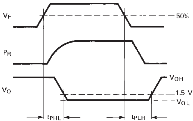
Figure 4: Propagation Delay Test Waveforms
