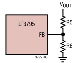
Figure 3. Feedback Resistor Connections for Boost and SEPIC Applications
