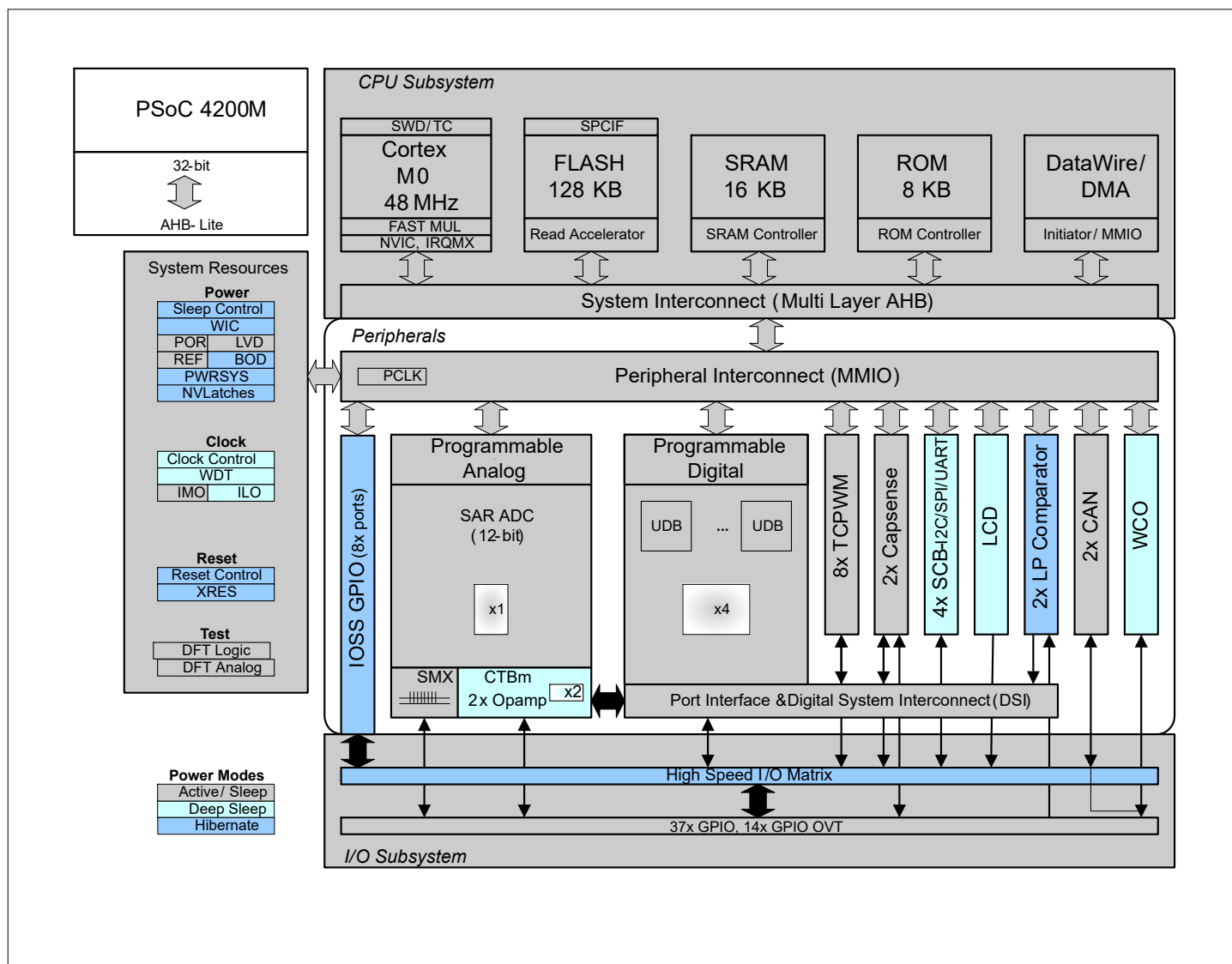
Figure 2 Block diagram
