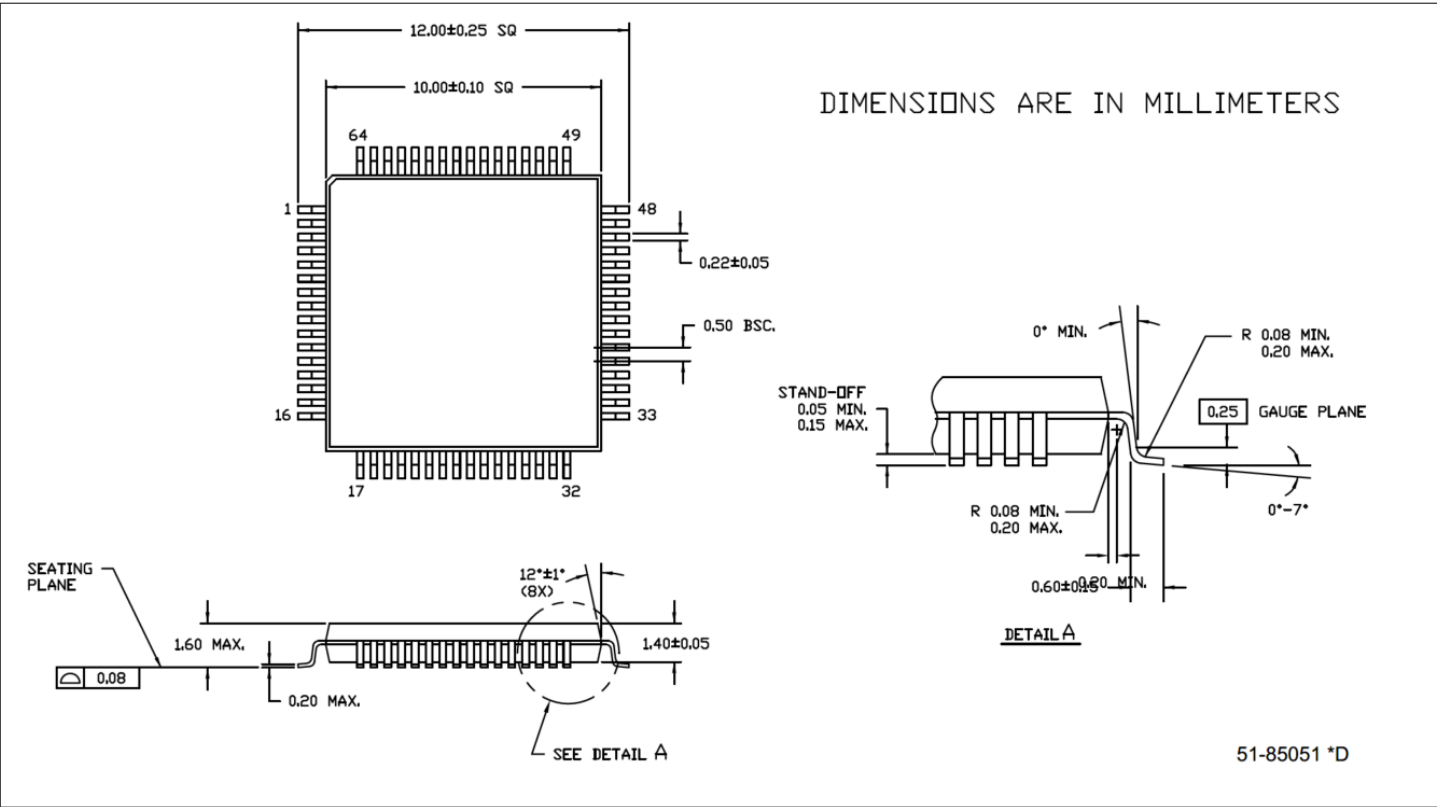
Figure 10 64-Pin TQFP 10 × 10 × 1.4 mm package outline (PG-TQFP-64)
