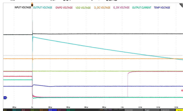
Figure 31. Shutdown by ON/PD ( I_{OUT} = 15\text{ A} , C_{OUT} = 6800 \mu F )
