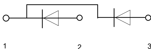
Circuit
