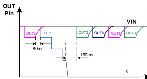
Figure 8: PD Plug into Port 2
