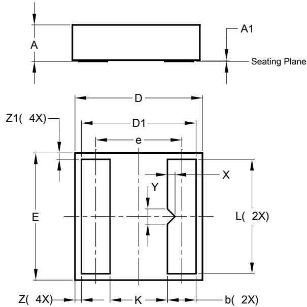
U-DFN2020-2
