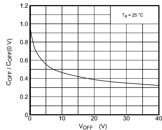
Fig. 12.1.10 C_{OFF}/C_{OFF}(0 V) - V_{OFF}
