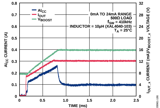
Figure 82. A_{I_{CC}} Current vs. Time for 24 mA Step Through 500 Ω Load with External 51 kΩ Compensation Resistor
