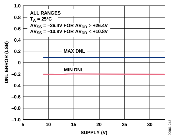
Figure 43. Differential Nonlinearity Error vs. Supply
