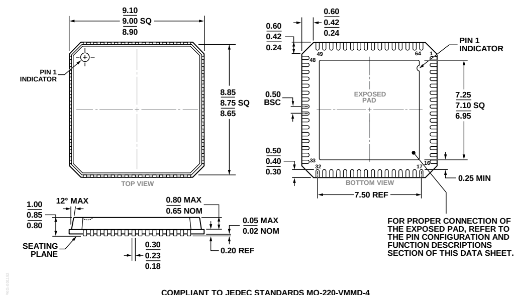
Figure 87. 64-Lead Lead Frame Chip Scale Package [LFCSP_VQ] 9 mm × 9 mm Body, Very Thin Quad (CP-64-3) Dimensions shown in millimeters
