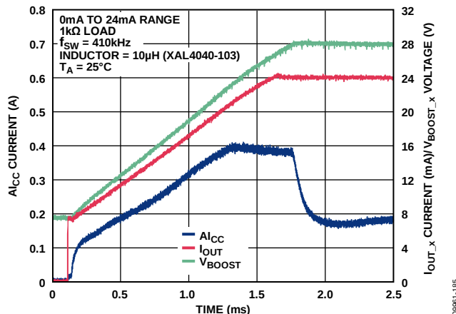
Figure 81. A_{I_{CC}} Current vs. Time for 24 mA Step Through 1 kΩ Load with External 51 kΩ Compensation Resistor
