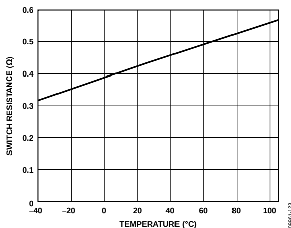
Figure 58. Switch Resistance vs. Temperature
