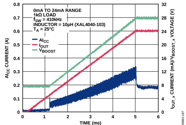
Figure 83. A_{I_{CC}} Current vs. Time for 24 mA Step Through 1 kΩ Load with Slew Rate Control
