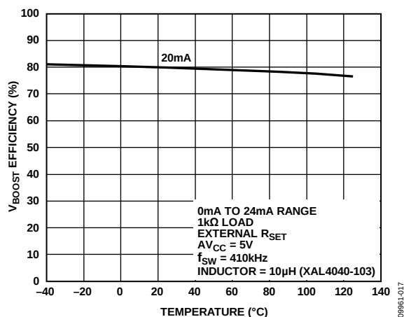
Figure 55. Efficiency at V_{BOOST\_X} vs. Temperature (See Figure 78)
