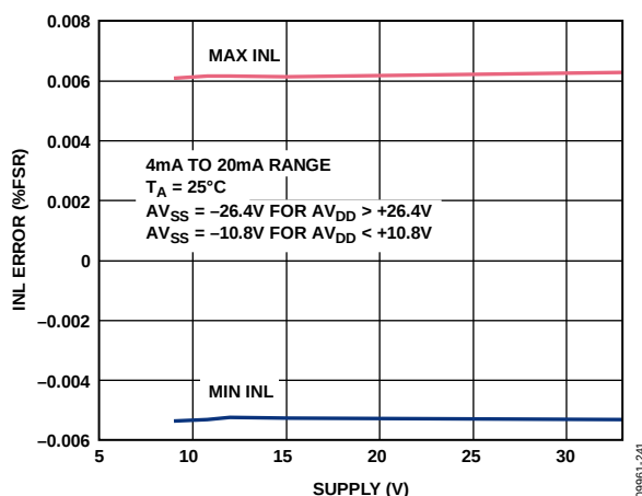
Figure 42. Integral Nonlinearity Error vs. Supply, Internal R_{SET}
