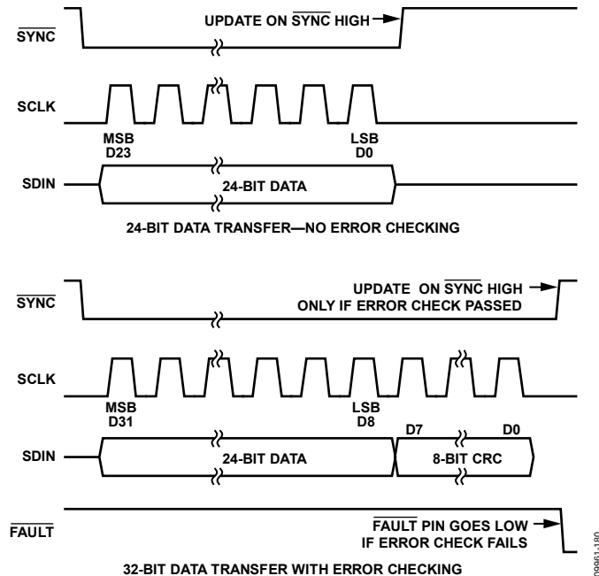
Figure 77. PEC Timing
