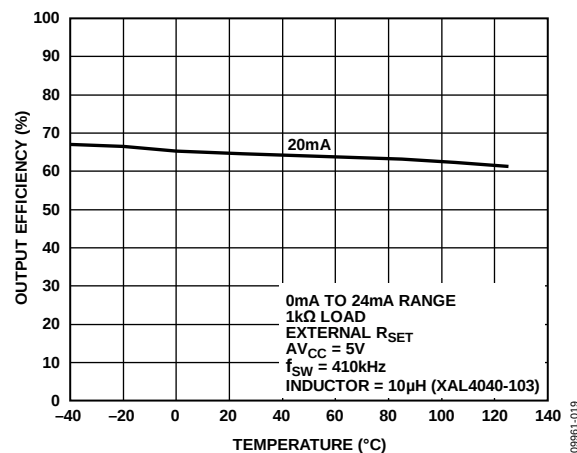
Figure 57. Output Efficiency vs. Temperature (See Figure 78)
