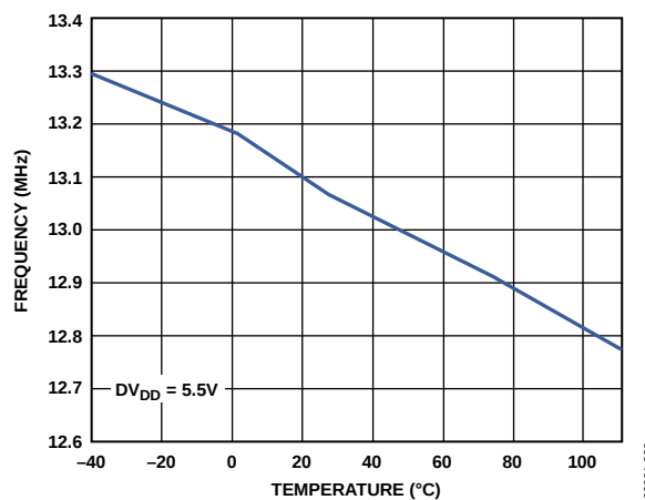
Figure 68. Internal Oscillator Frequency vs. Temperature
