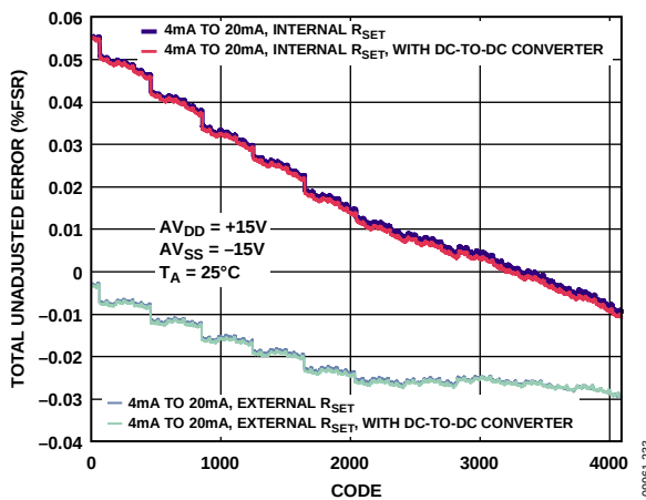
Figure 34. Total Unadjusted Error vs. DAC Code
