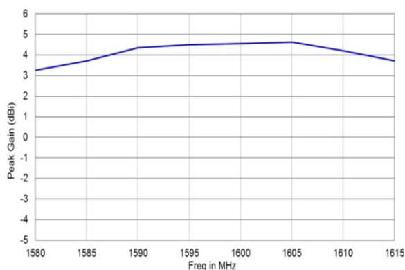
Peak Gain
