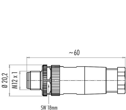
Scale drawing
