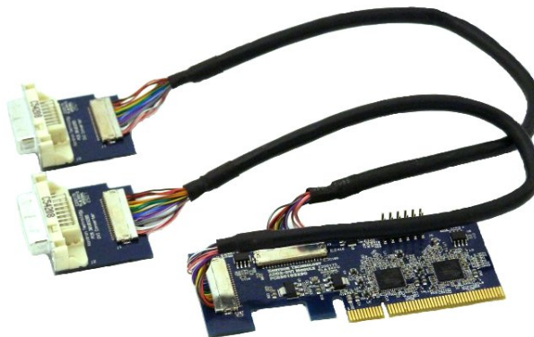
Example: 820951 ADD2-DVI-Dual-Internal with cables mounted.
