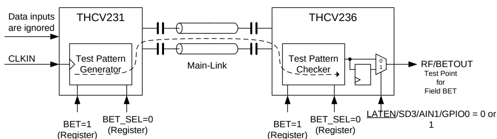
Figure 3. Main-Link Field BET Configuration
