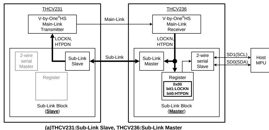
Figure 2. HTPDN, LOCKN transmission route
