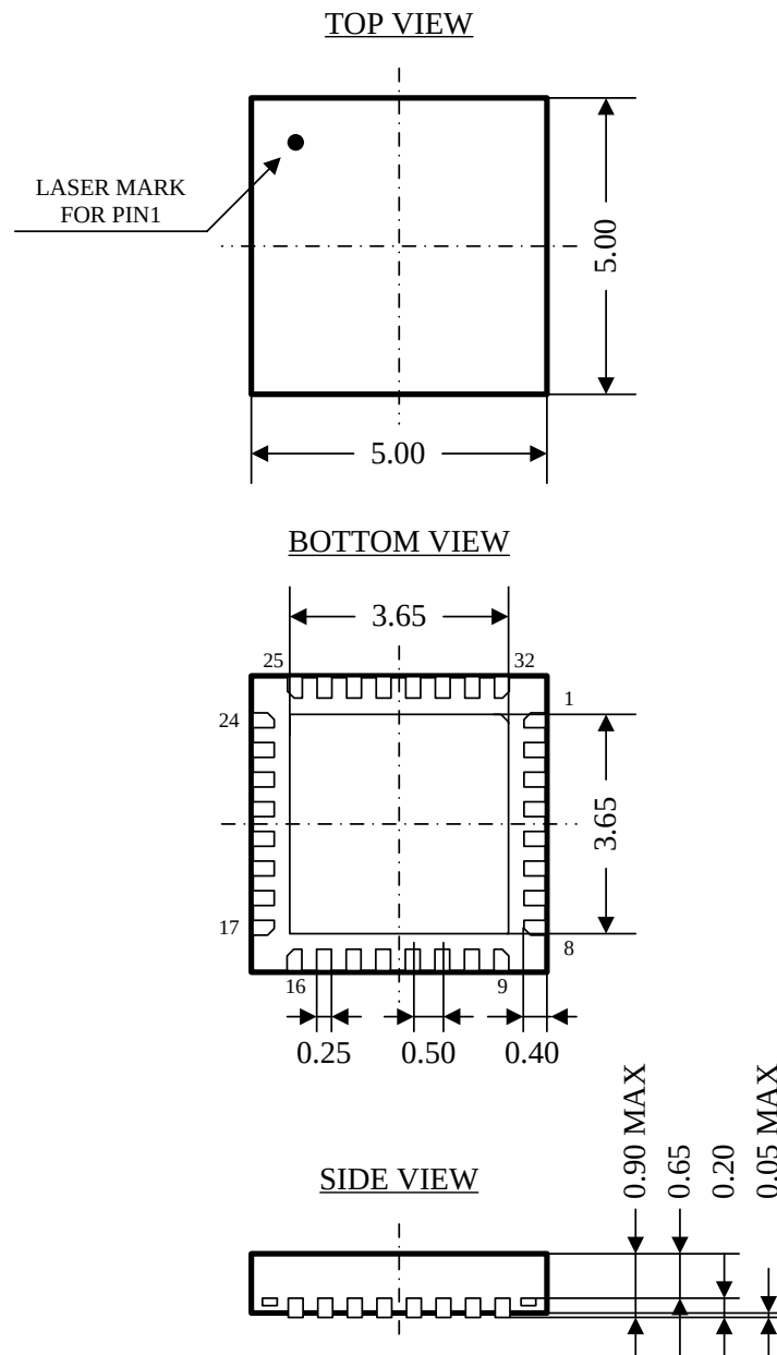
Figure 35. 32-pin QFN package physical dimension
