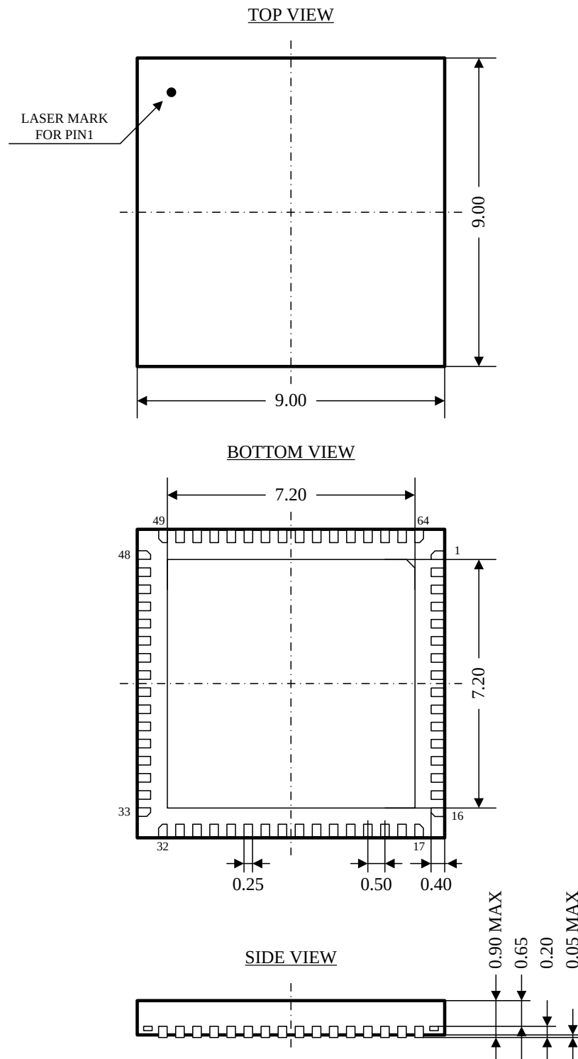
Figure 36. 64-pin QFN package physical dimension
