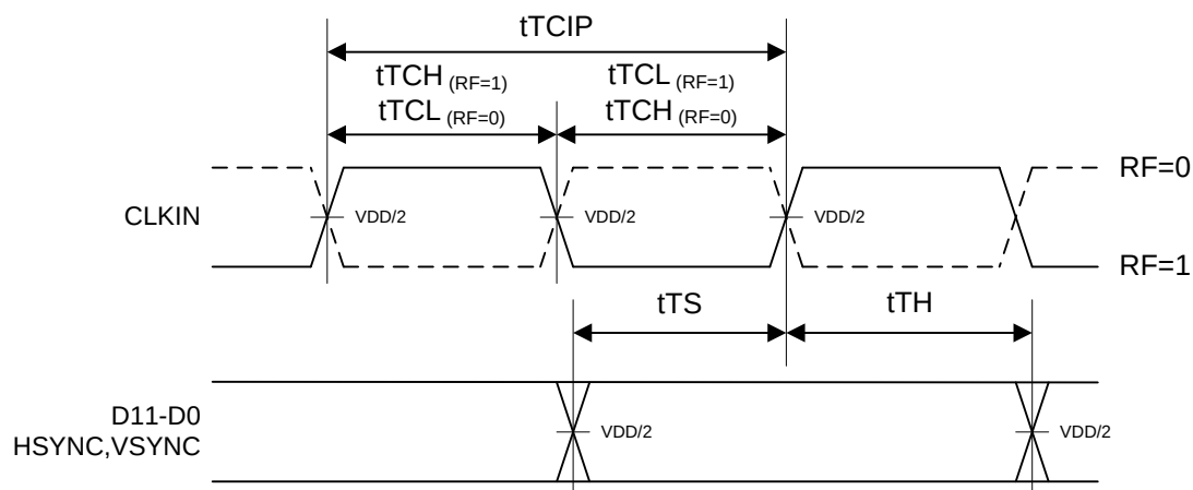
Figure 15. LVC MOS Input Switching Timing Diagrams
