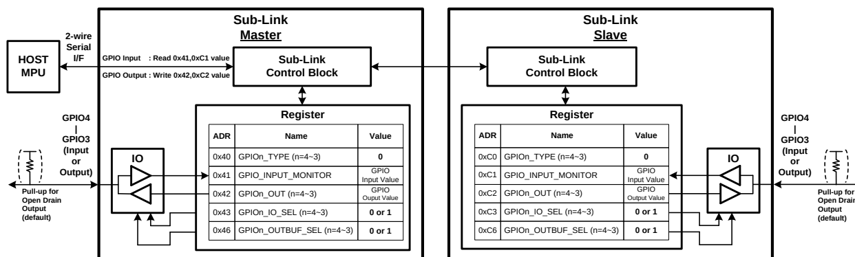
Figure 12. Programmable GPIO
