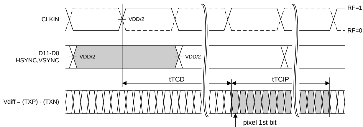
Figure 20. THCV231 Latency
