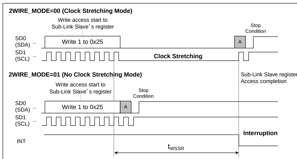
Figure 25. Write access completion time to Sub-Link Slave register
