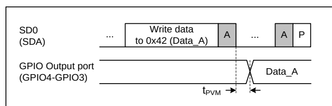
Figure 31. Programmable GPIO output timing at Sub-Link Master side
