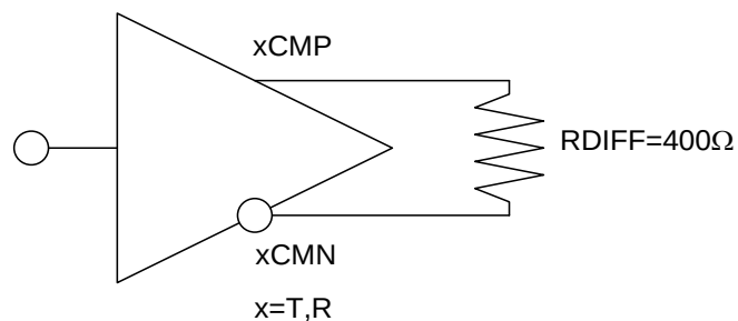
Figure 19. Bi-directional CML VBOD/VBOC Test Circuit
