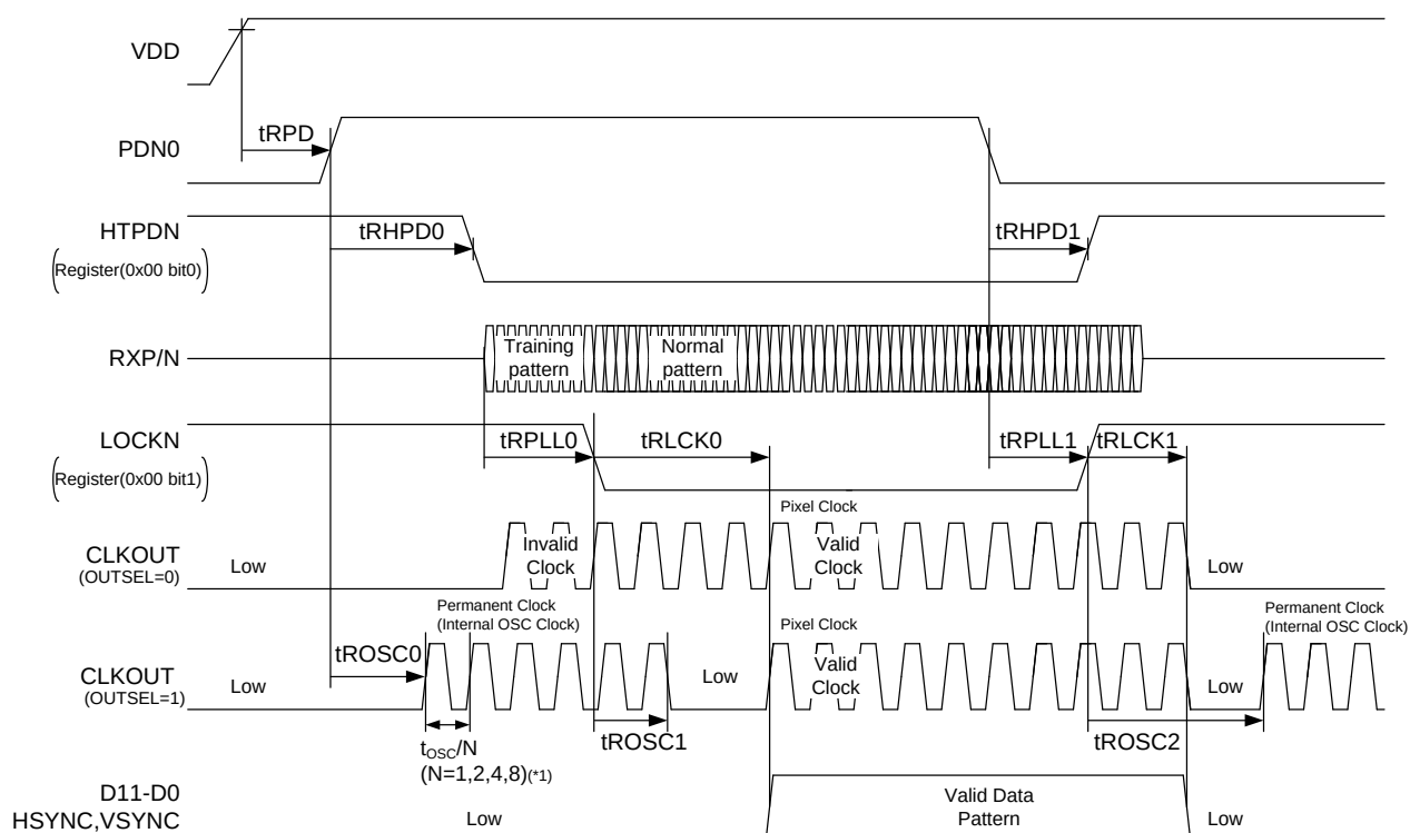
Figure 22. THCV231 Lock/Unlock Sequence
