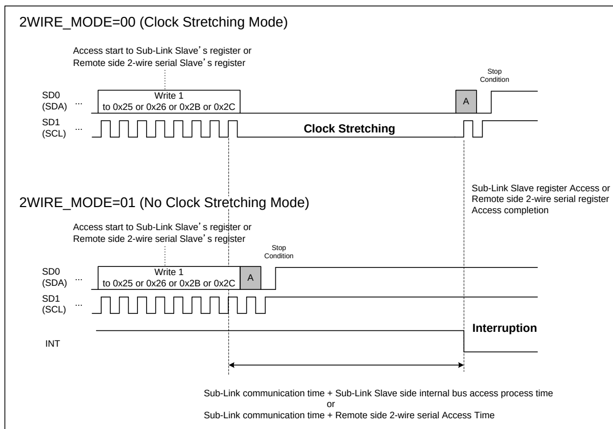
Figure 5. 2WIRE_MODE Operation
