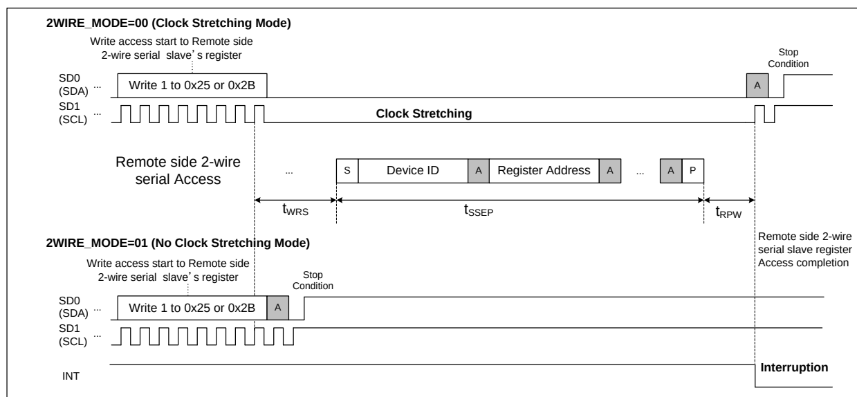
Figure 27. Write access completion time to Remote side 2-wire serial slave register
