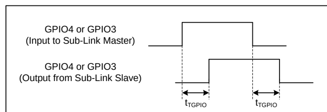
Figure 29. Through GPIO delay
