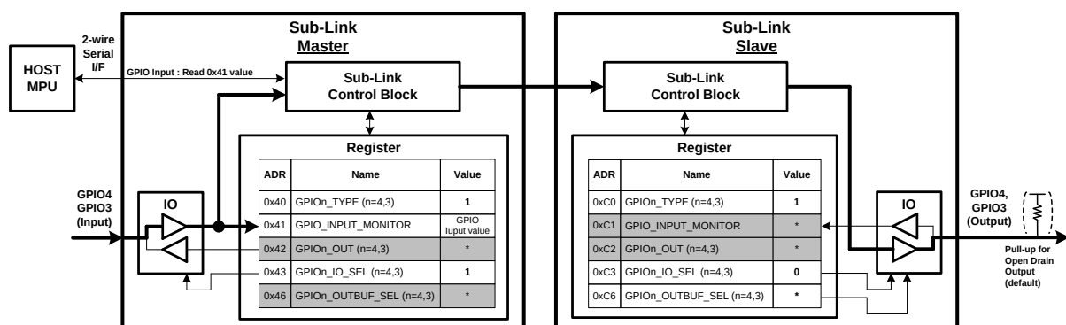
Figure 11. Through GPIO
