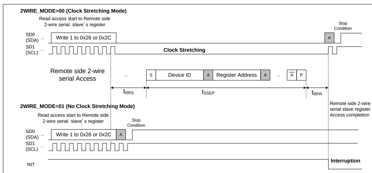
Figure 28. Read access completion time to Remote side 2-wire serial slave register
