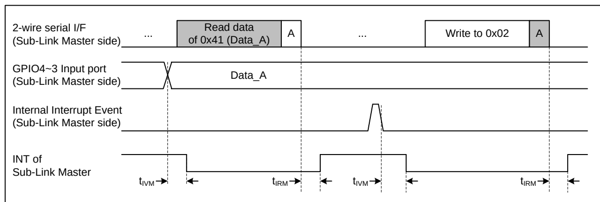
Figure 33. GPIO input and other interrupt event timing at Sub-Link Master side
