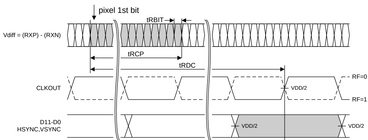
Figure 21. THCV236 Latency
