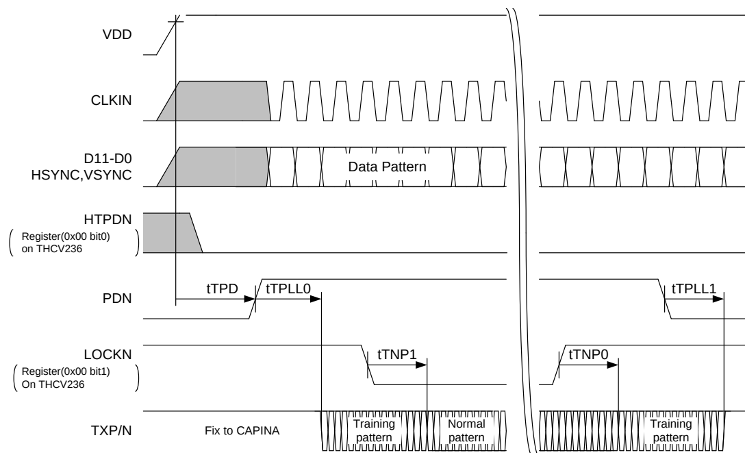
Figure 22. THCV231 Lock/Unlock Sequence
