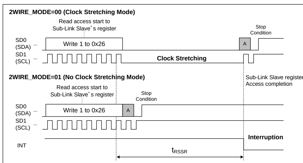
Figure 26. Read access completion time to Sub-Link Slave register
