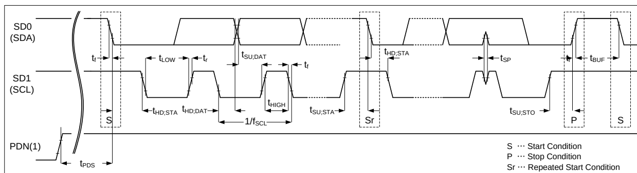
Figure 24. 2-wire serial interface Timing Diagram
