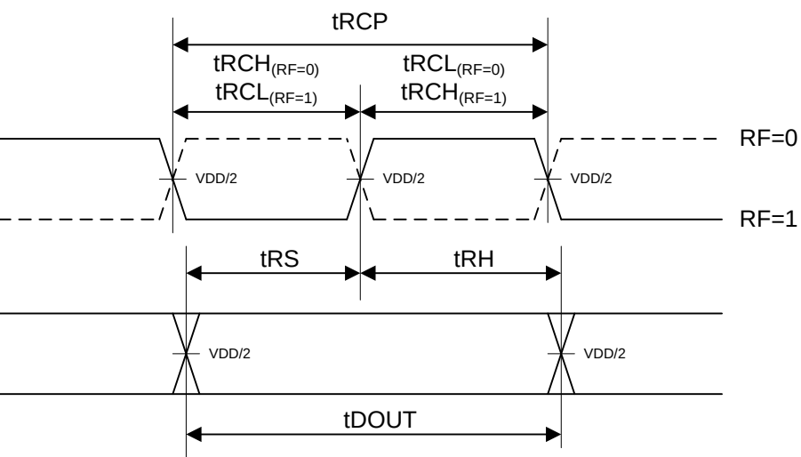
Figure 16. LVC MOS Output Switching Timing Diagrams
