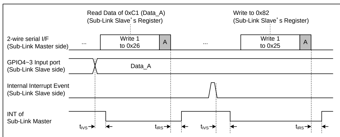
Figure 34. GPIO input and other interrupt event timing at Sub-Link Slave side
