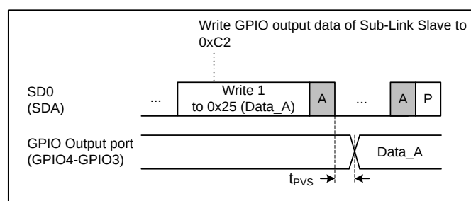
Figure 32. Programmable GPIO output timing at Sub-Link Slave side
