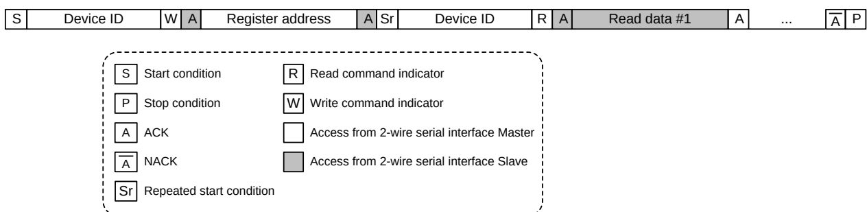
Figure 8. 2-wire serial I/F read to Sub-Link Master register protocol
