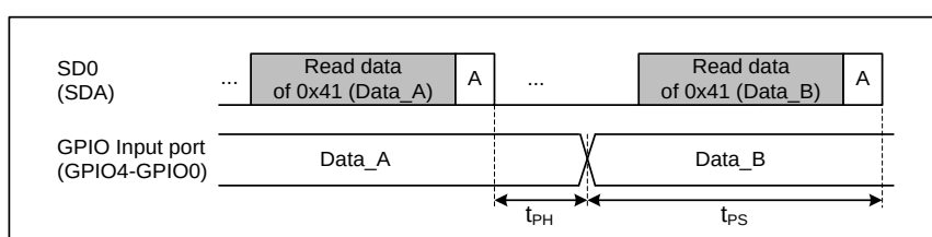
Figure 30. Programmable GPIO input timing at Sub-Link Master side
