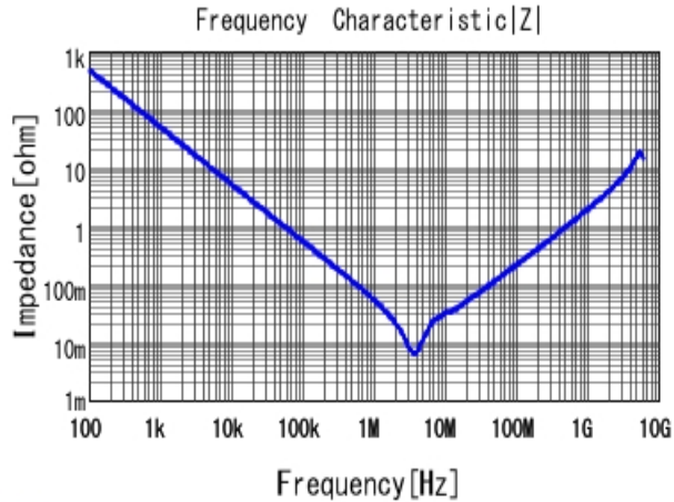
■ GRM219R61C475KE15 |Z| DC0V, 25degC
