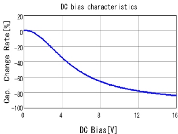
■ GRM219R61C475KE15 C-DC bias capchange, 25.0degC, AC0.
