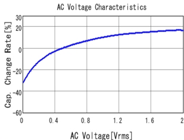
■ GRM219R61C475KE15 C-AC Voltage capchange, DC0V, 25.0d
