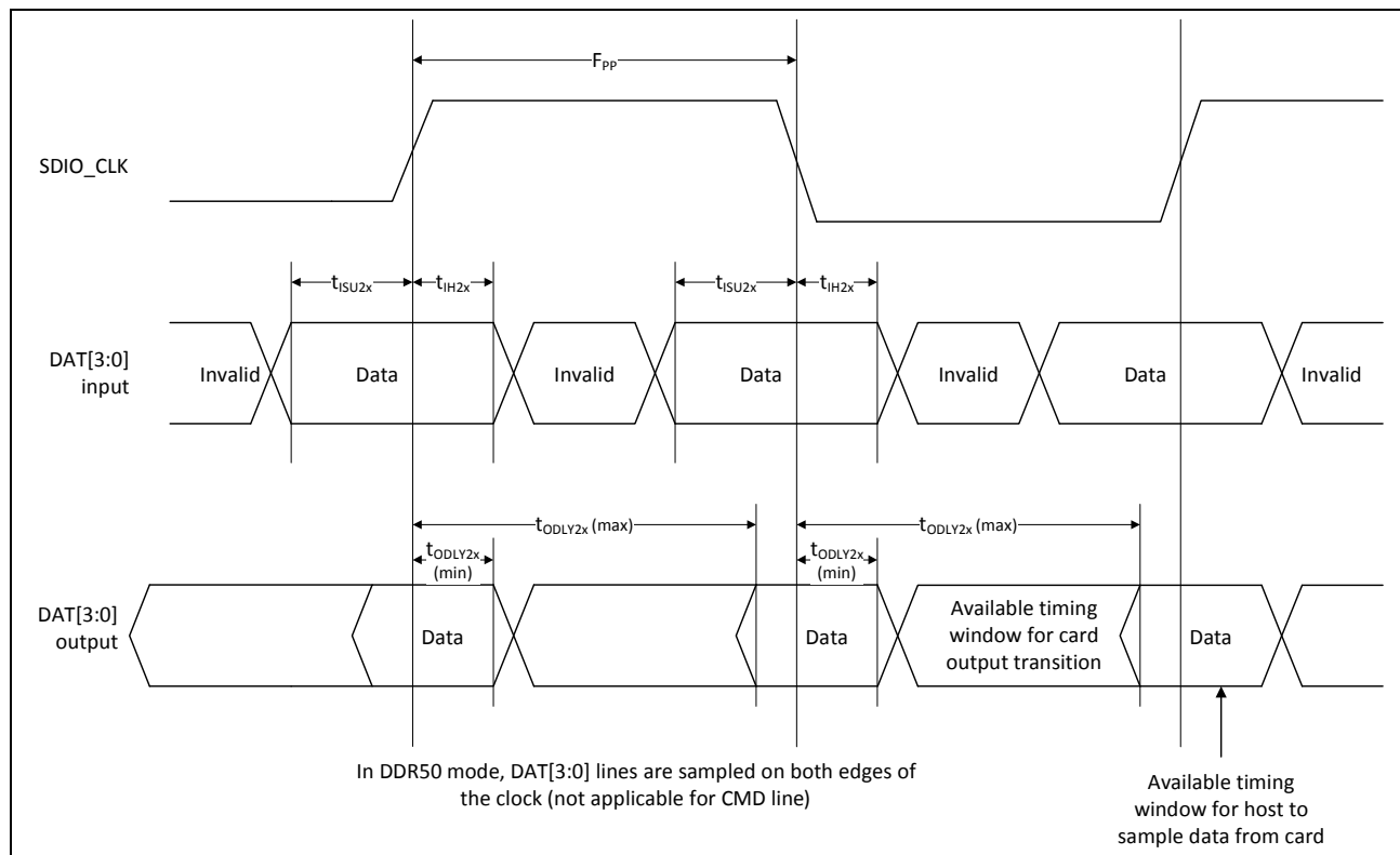
Figure 41: SDIO Data Timing (DDR50 Mode)
