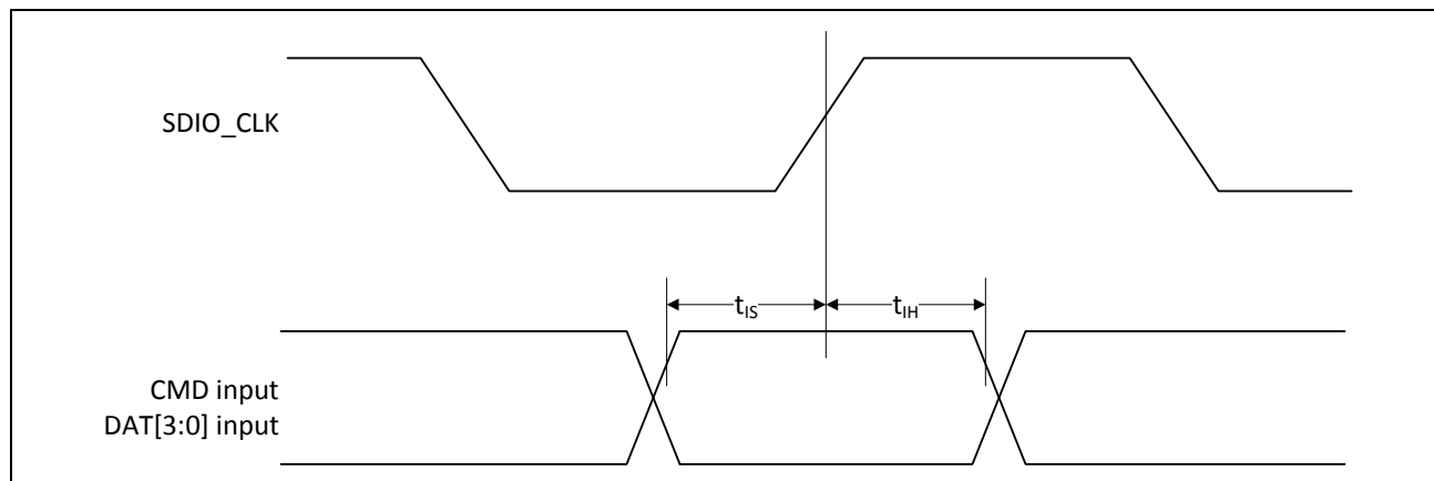
Figure 36: SDIO Bus Input Timing (SDR Modes)
