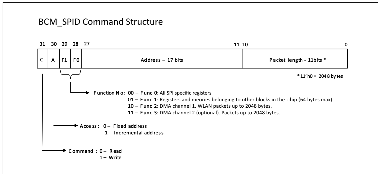
Figure 23: gSPI Command Structure
