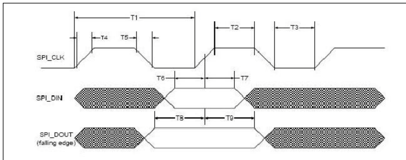
Figure 42: gSPI Timing
