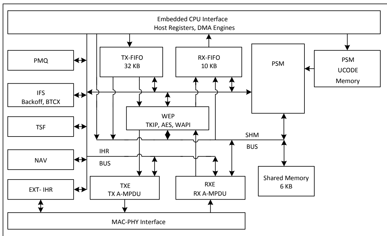
Figure 27: WLAN MAC Architecture
