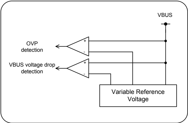
Figure 4-3 Voltage Detection Block Diagram
