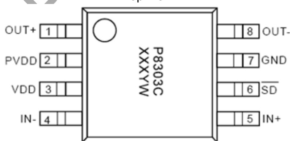
MSOP-8(B) Top View
