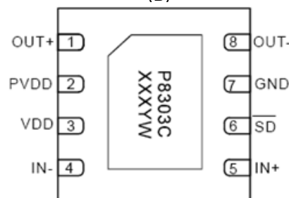
U-DFN3030-8 (B)
