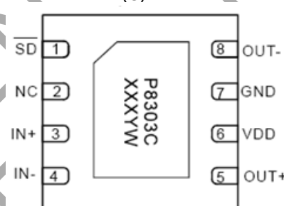
U-DFN3030-8 (C)
