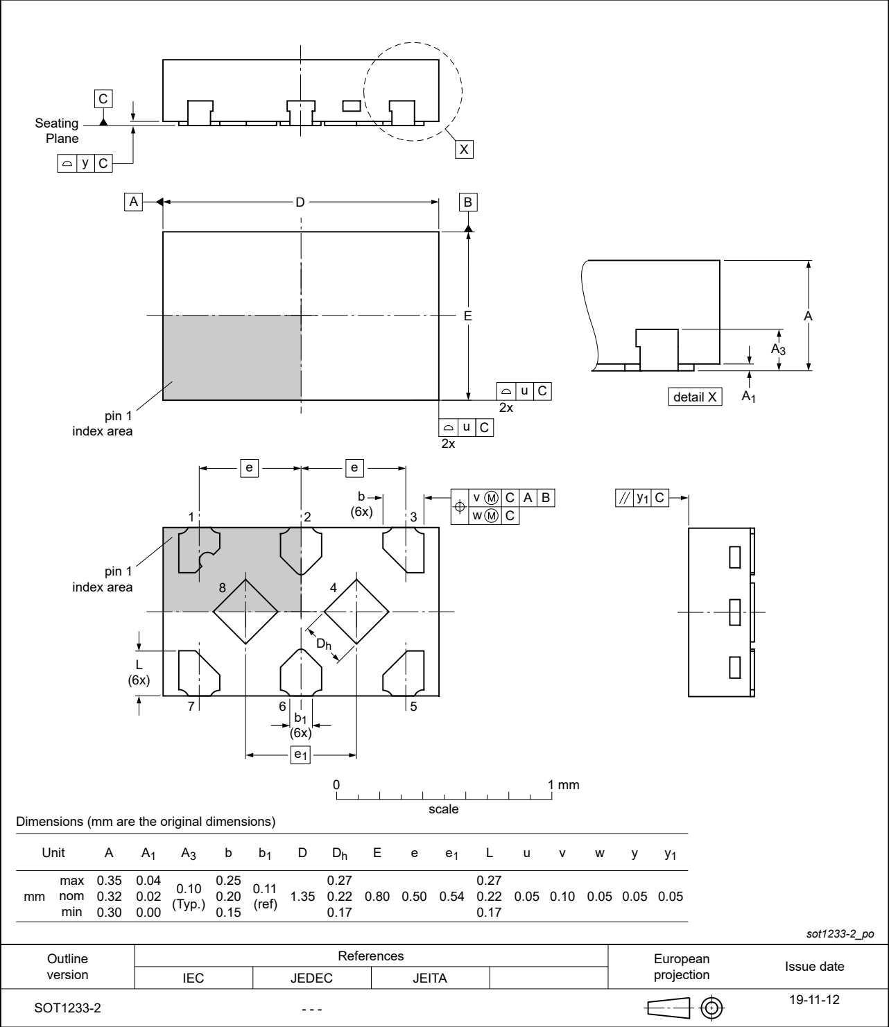
Fig. 17. Package outline SOT1233-2 (X2SON8)
