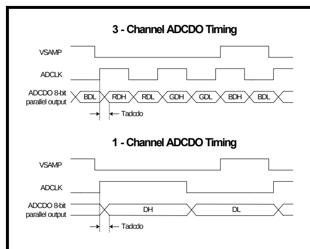
FIGURE 5. ADCDO TIMING (ADCLK POL =0, VSAMP POL =0)
