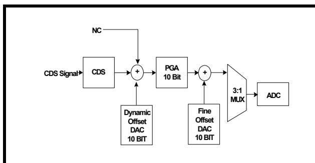
FIGURE 6. CDS TO ADC SIGNAL PATH
