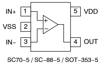
Single Channel Configuration NCS21871, NCV21871
