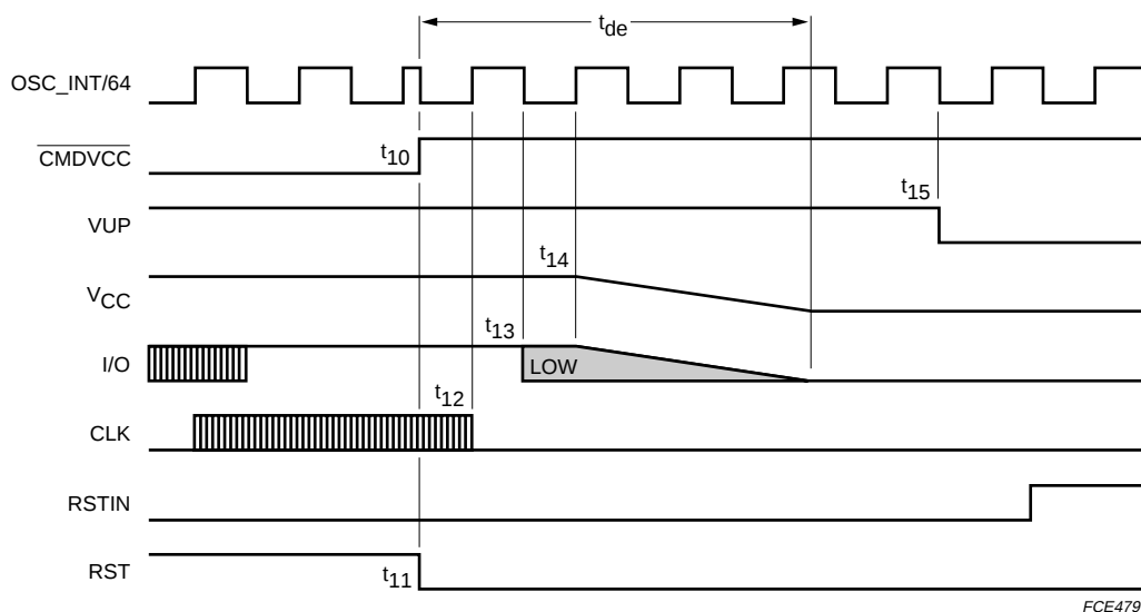
Fig.13 Deactivation sequence
