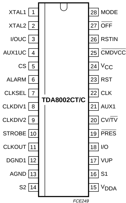
Fig.4 Pin configuration (TDA8002CT/C).
