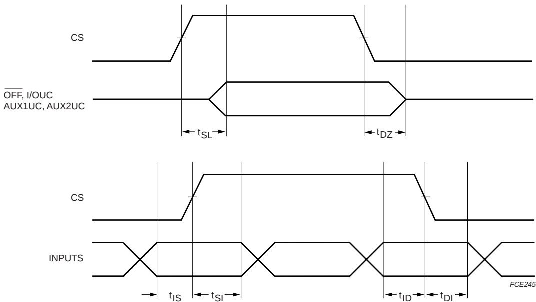
Fig.7 Chip select.
