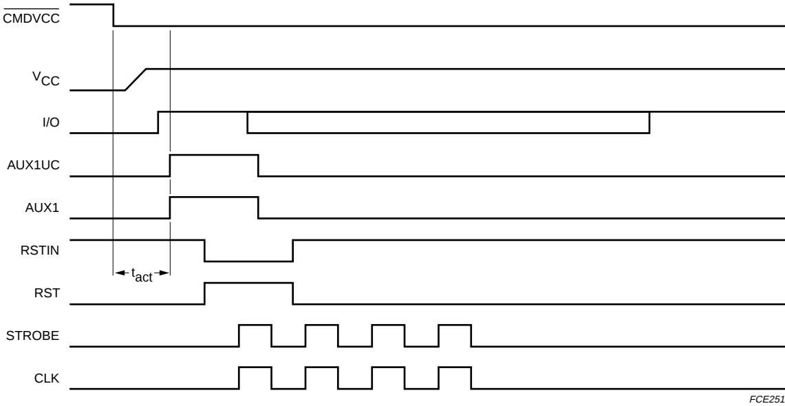
Fig.12 Activation sequence for synchronous application.
