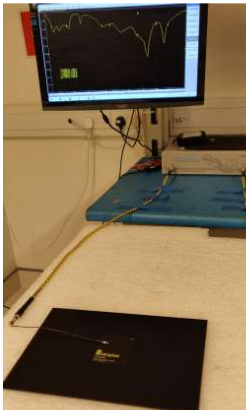
VNA Set-Up
