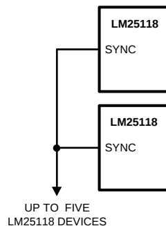
Figure 12. Sync from Multiple Devices
