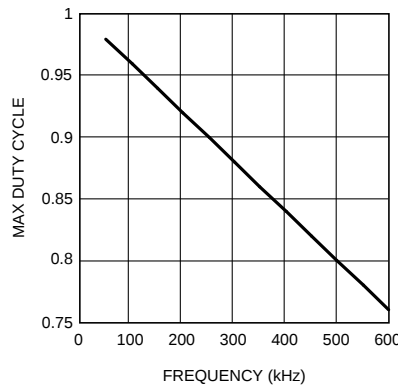
Figure 16. Maximum Duty Cycle vs Frequency
