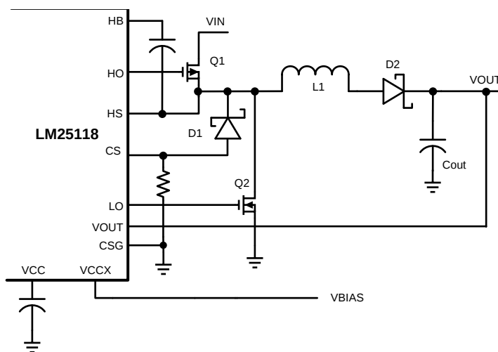
Figure 29. VCC Bias with Additional Bias Supply
