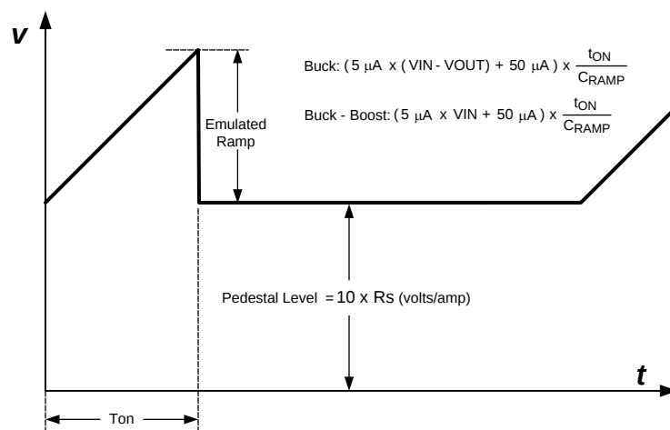
Figure 14. Composition of Emulated Current Signal
