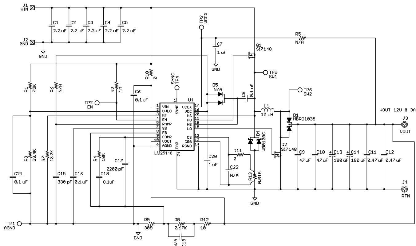
Figure 20. 12 V, 3 A Typical Application Schematic
