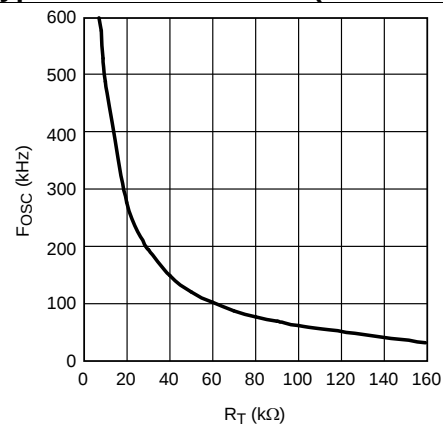
Figure 8. Oscillator Frequency vs R_T
