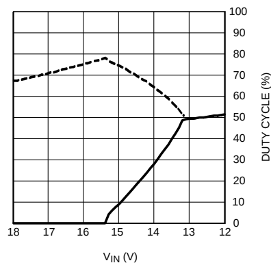
Figure 11. Mode Dependence on Duty Cycle ( V_{OUT} = 12\text{ V} )
