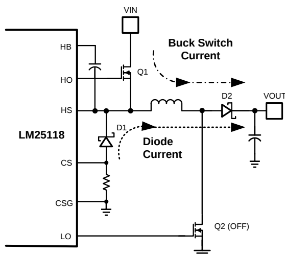
Figure 9. Buck Mode Operation
