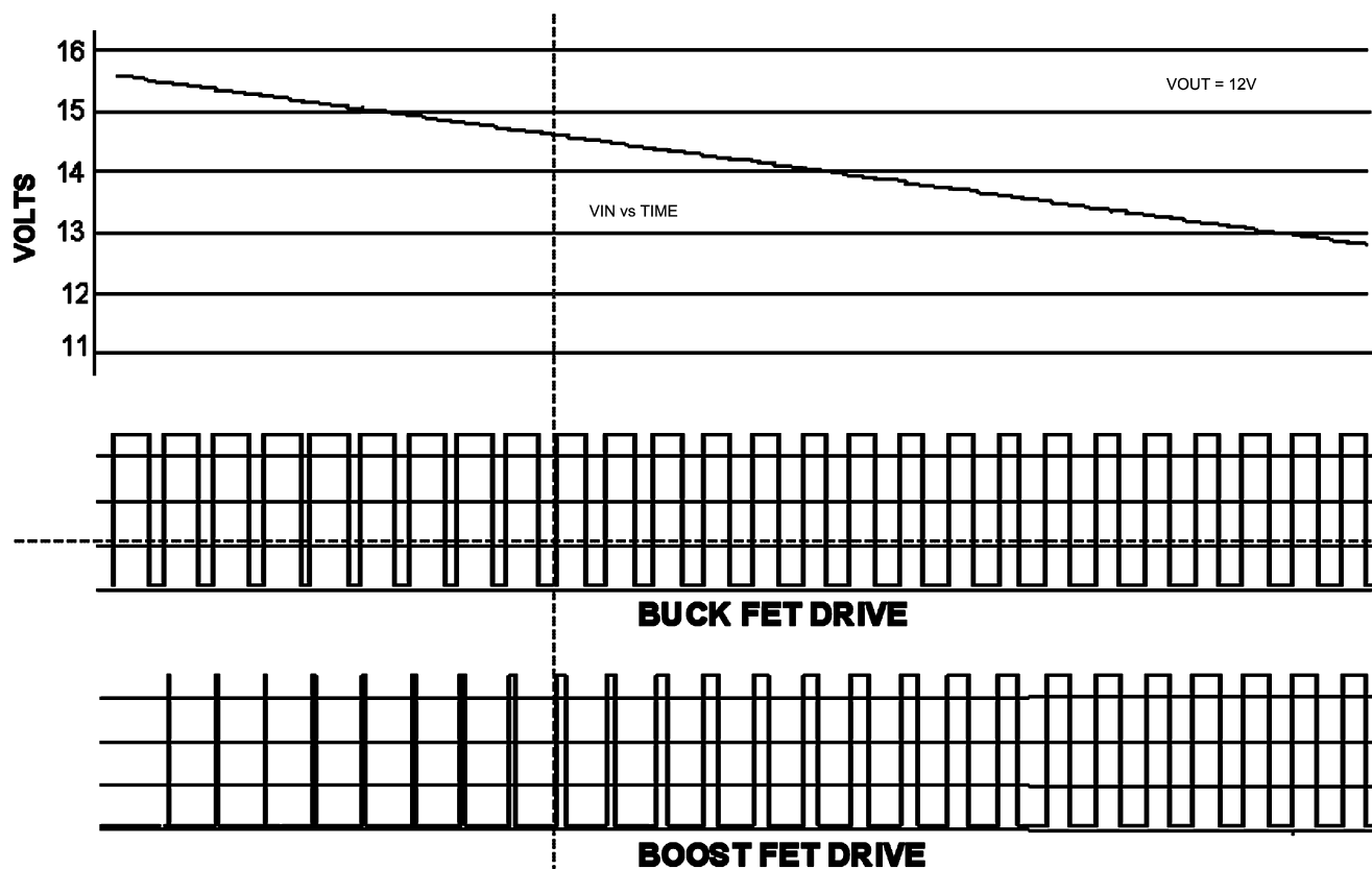
Figure 17. Buck (HO) and Boost (LO) Switch Duty Cycle vs. Time, Illustrating Gradual Mode Change with Decreasing Input Voltage
