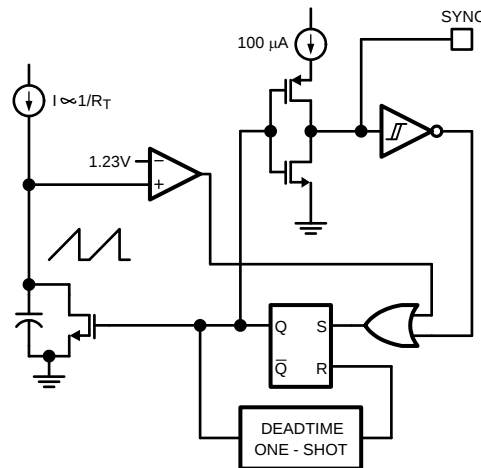
Figure 13. Simplified Oscillator and Block Diagram with Sync I/O Circuit
