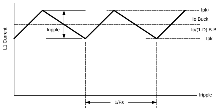
Figure 21. Inductor Current Waveform
