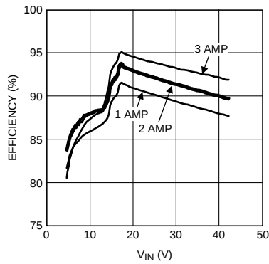
Figure 2. Efficiency vs VIN and IOUT VOUT = 12 V
