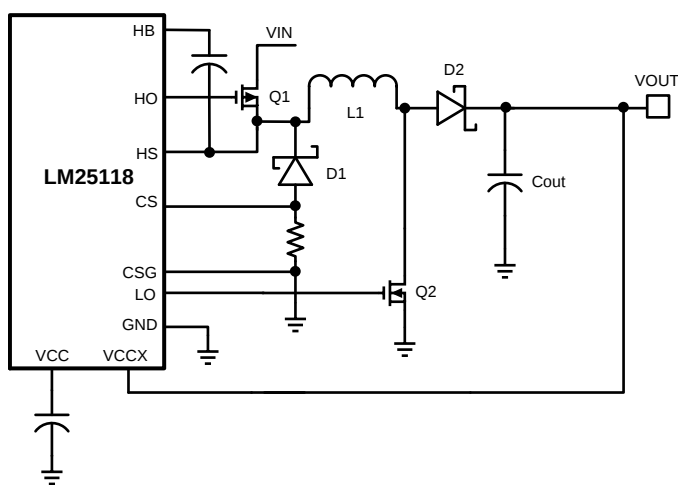
Figure 28. VCC Bias from VOUT 4 V < VOUT < 15 V
