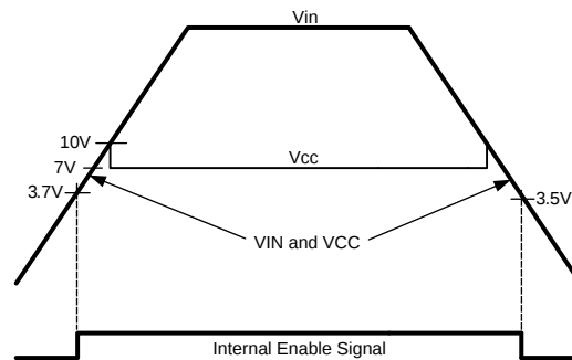
Figure 18. VIN and VCC Sequencing
