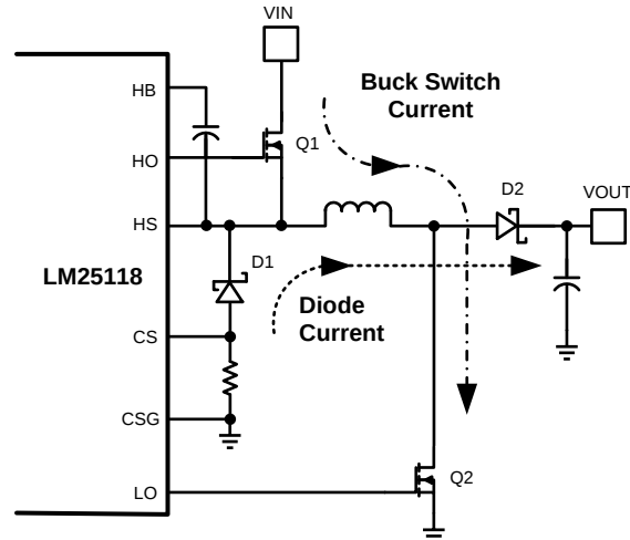
Figure 10. Buck-Boost Mode Operation
