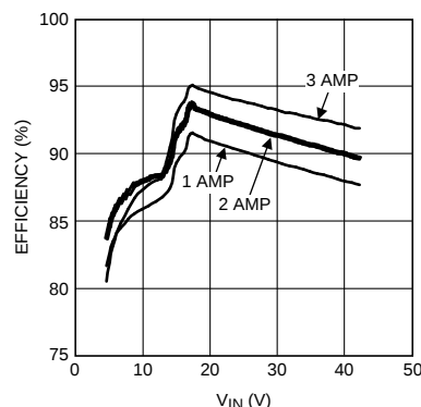
Figure 1. Efficiency vs VIN and IOUT VOUT = 12 V
