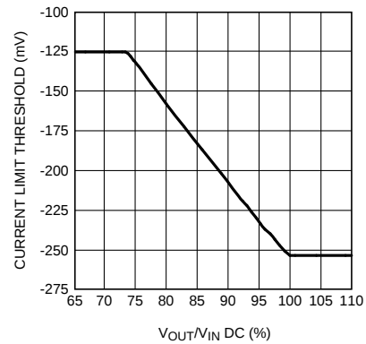
Figure 3. Current Limit Threshold vs VOUT/VIN VOUT = 12 V
