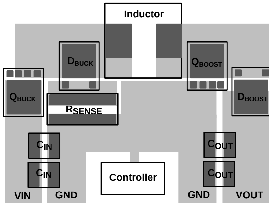
Figure 30. LM25118(Q1) Layout Example
