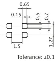
Recommended mounting pad ( TOP VIEW )
