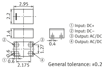
External dimensions
