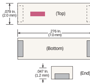
Case 43-1
