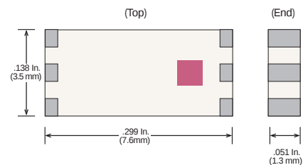
Case 44-1
