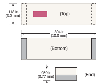
Case 47-1
