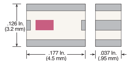
Case 44-1
