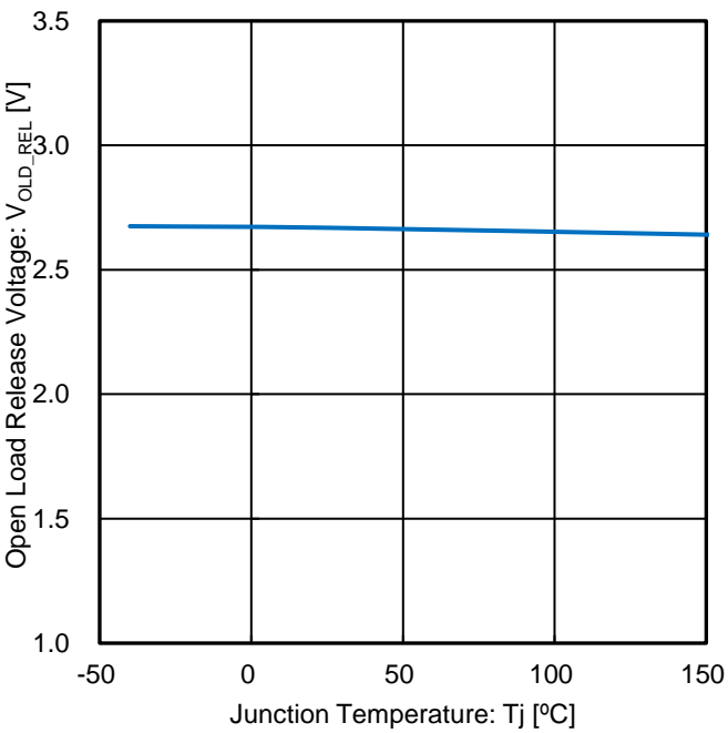
Figure 39. Open Load Release Voltage vs Junction Temperature
