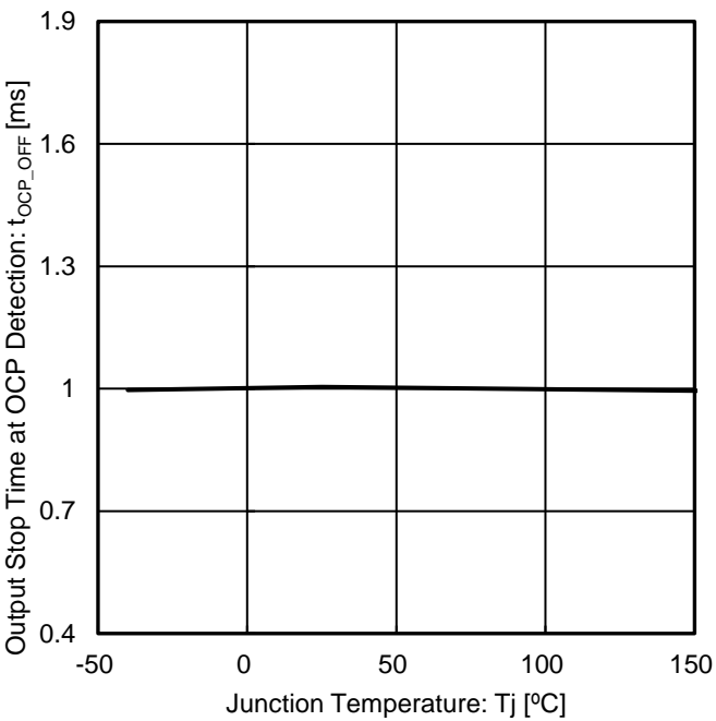
Figure 37. Output Stop Time at OCP Detection vs Junction Temperature
