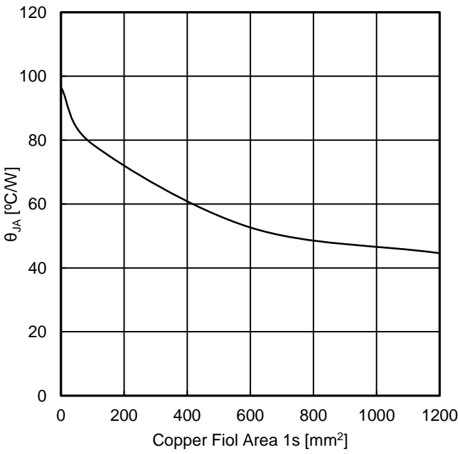
Figure 7. Thermal Resistance
