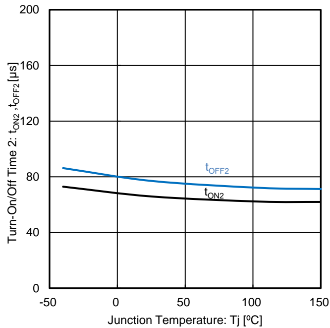
Figure 29. Turn-On/Off Time 2 vs Junction Temperature
