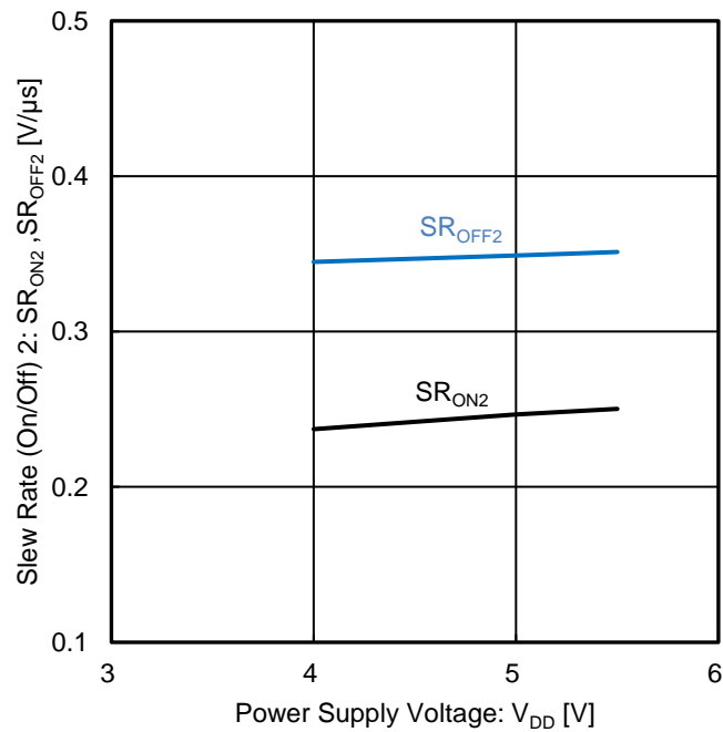
Figure 30. Slew Rate (On/Off) 2 vs Power Supply Voltage
