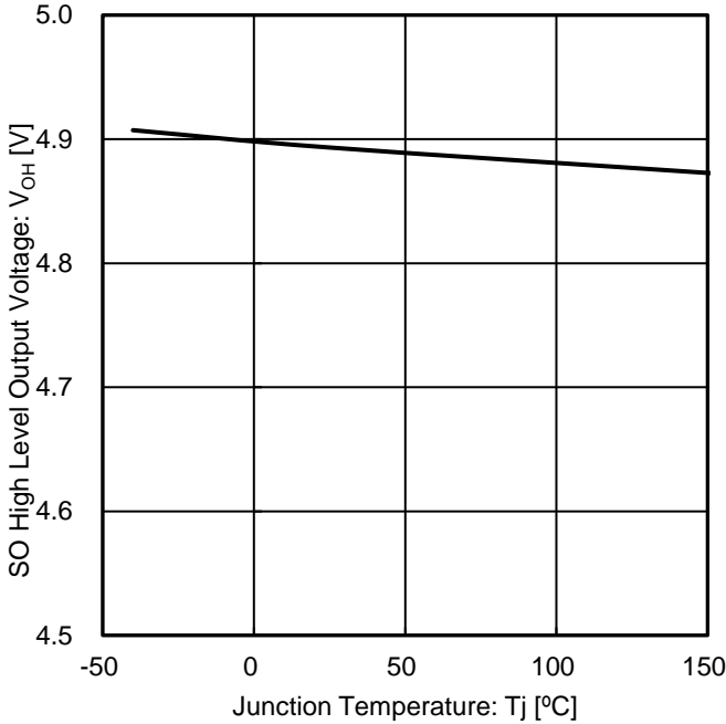
Figure 17. SO High Level Output Voltage vs Junction Temperature
