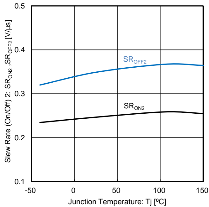
Figure 31. Slew Rate (On/Off) 2 vs Junction Temperature
