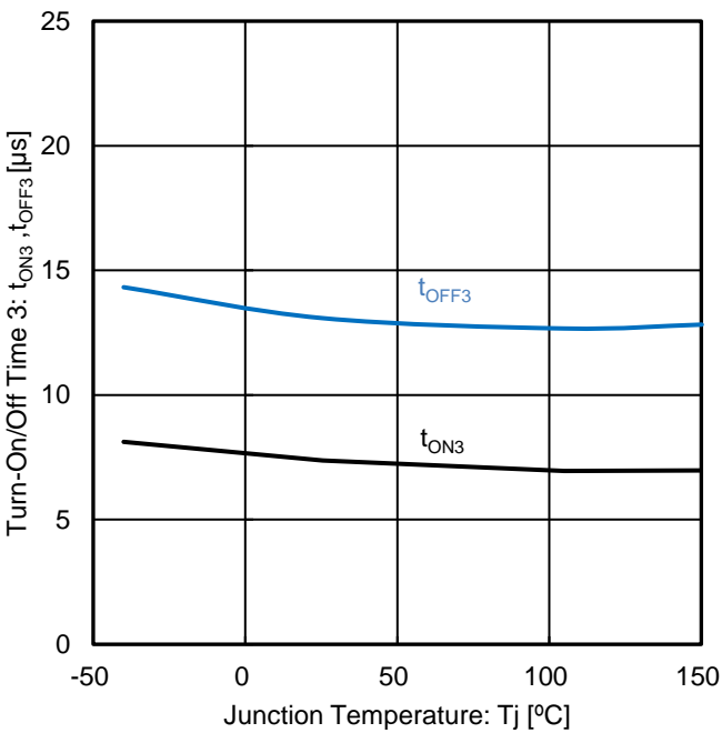
Figure 33. Turn-On/Off Time 3 vs Junction Temperature
