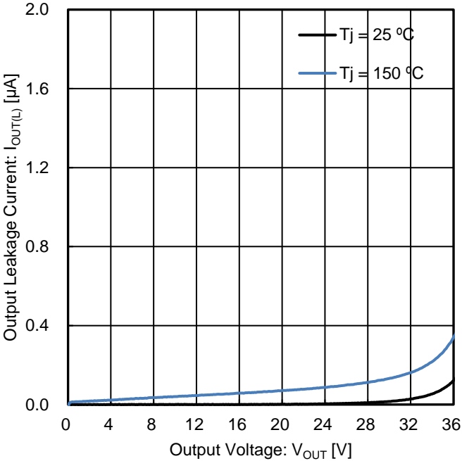
Figure 21. Output Leakage Current vs Output Voltage
