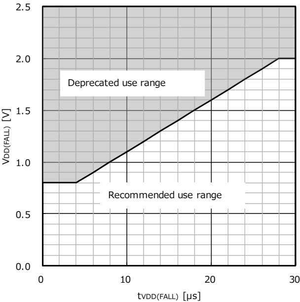
Figure 56. Recommended use range
