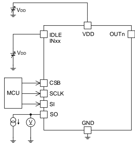
Figure 50. SO High/Low Level Output Voltage
