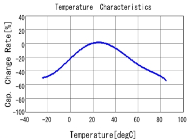
■ DE2E3SA222MN3AY02F C-Temp. capchange, DCOV, AC1Vrms
