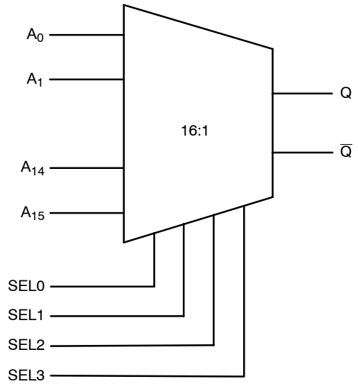
Figure 2. Logic Diagram
