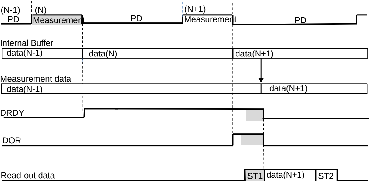
Figure 11.8. Skipping Data
