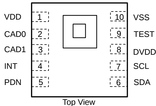
Figure 5.1 Pin Configurations
