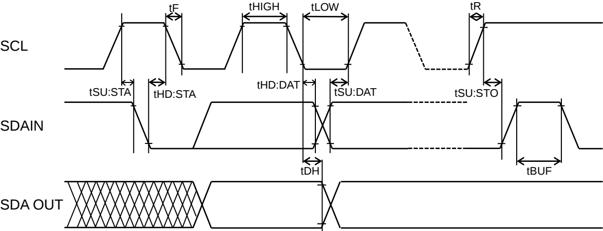
Figure 10.1. Bus Timing
