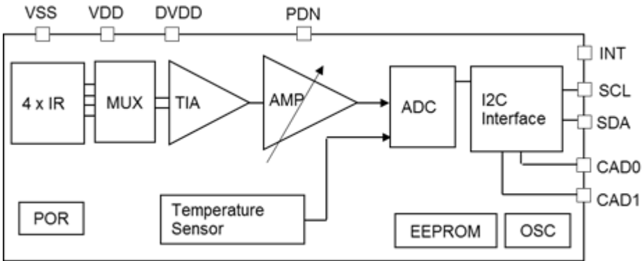
Figure 4.1 AK9750 Block Diagram
