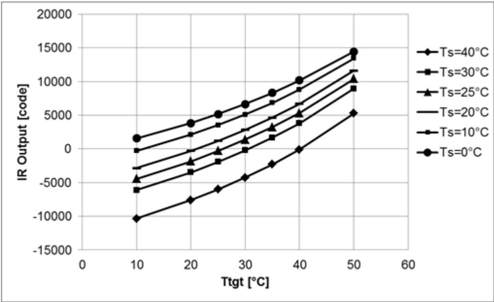
Figure 18.1. IR Output
