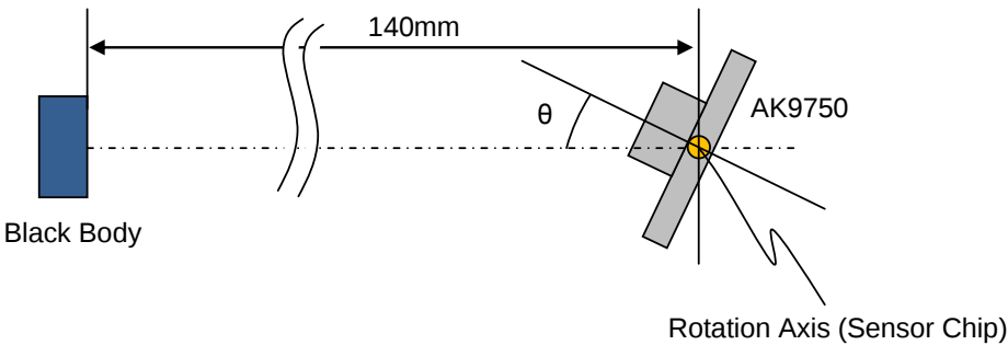
Figure 20.2. Measurement Conditions
