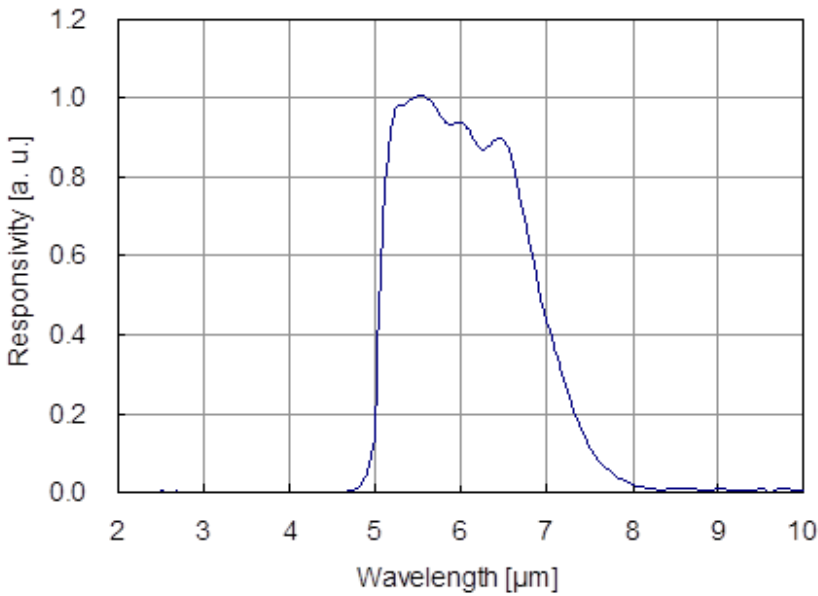
Figure 19.1. Spectrum Sensitivity
