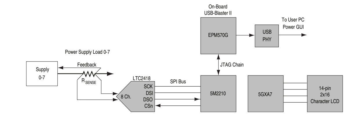
Figure 2-11. Power Measurement Circuit
