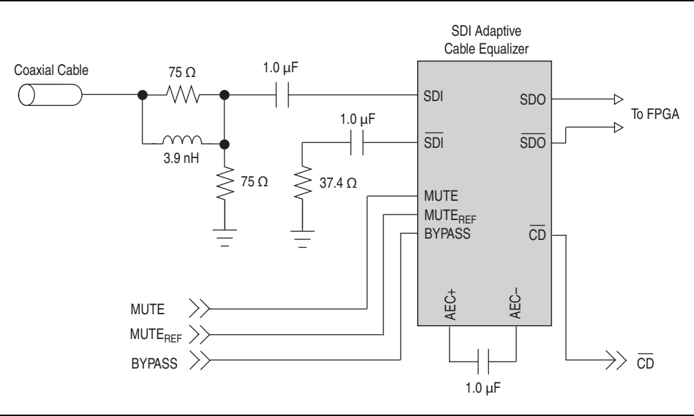
Figure 2-9. SDI Cable Equalizer
