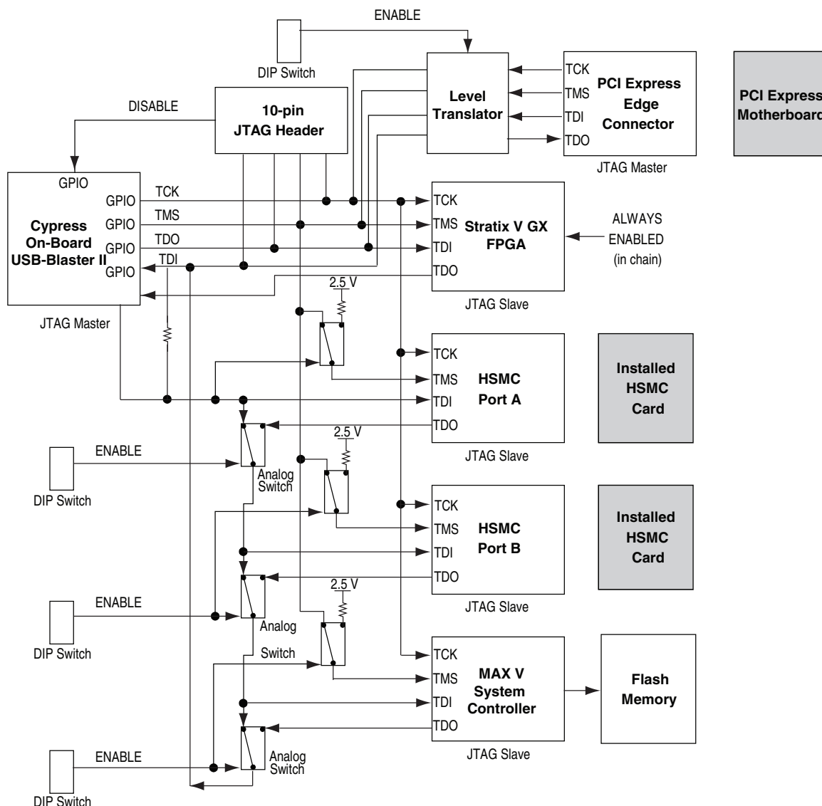
Figure 2-3. JTAG Chain
