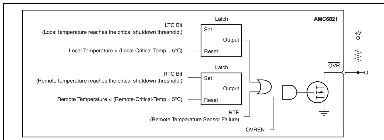
Figure 30. \overline{\text{OVR}} Pin
