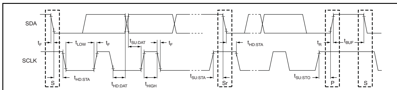
Figure 1. Timing Specification
