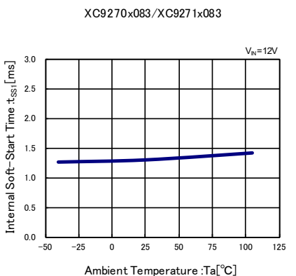
(14) Internal Soft-Start Time vs. Ambient Temperature
