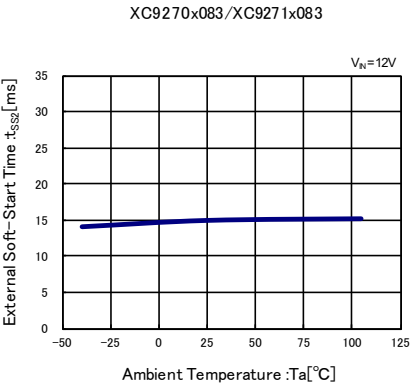
(15) External Soft-Start Time vs. Ambient Temperature
