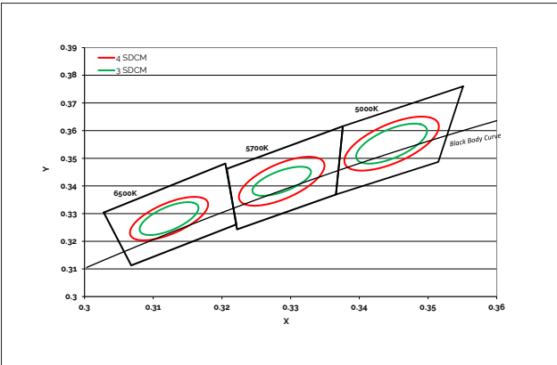
Figure 20: Cool White Test Bins in xy Color Space
