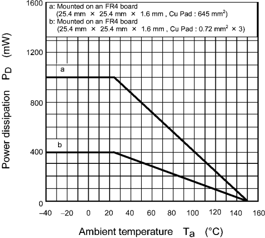
Fig. 8.12 P_D - T_a
