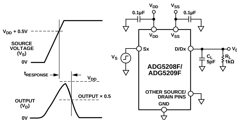
Figure 43. Overvoltage Response Time, t_{\text{RESPONSE}}
