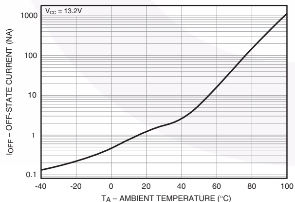
Fig. 12 Off-State Current vs. Ambient Temperature
