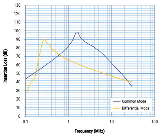
GTX-3600-Y104
