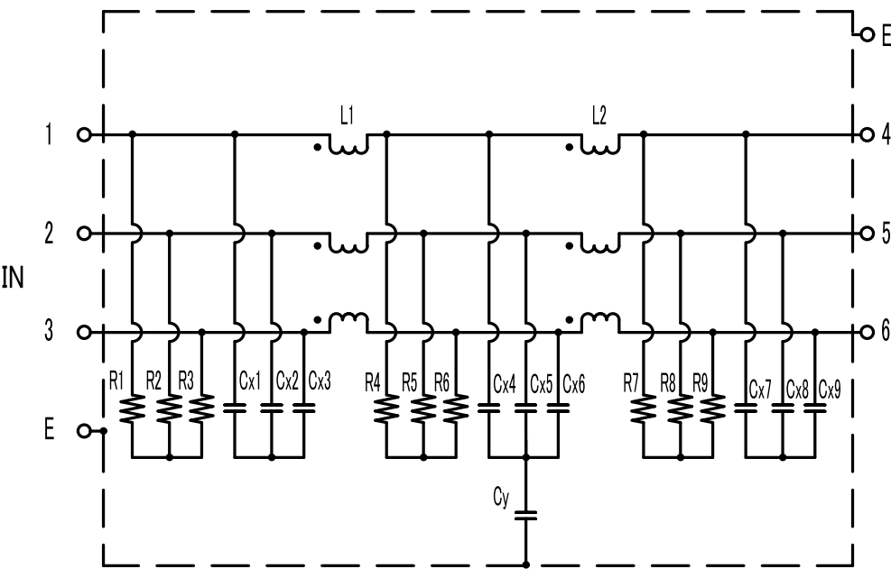
Measuring Circuit - Common Mode
