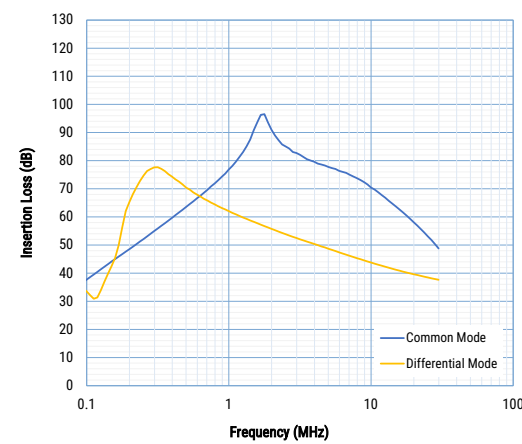
GTX-3800-Y683
