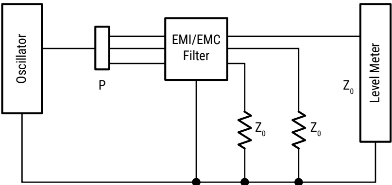
Measuring Circuit - Common Mode
