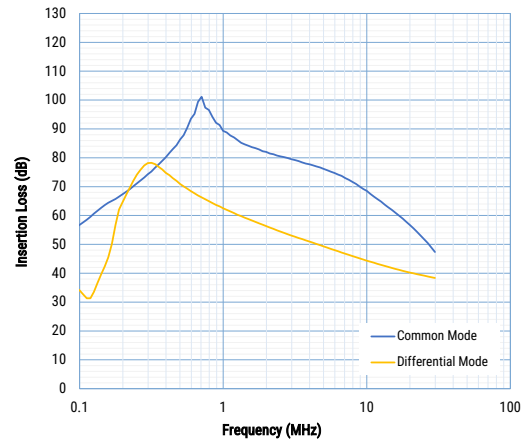
GTX-3800-Y474
