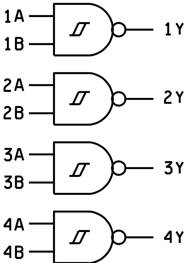
FIGURE 3. Logic diagram.
