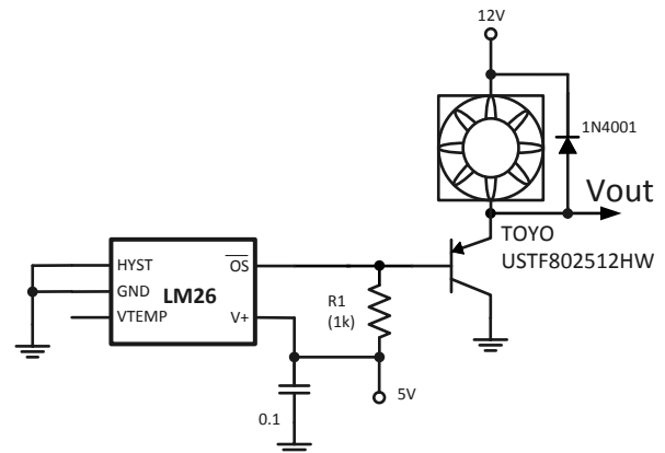
Figure 11. Fan Low-Side Drive
