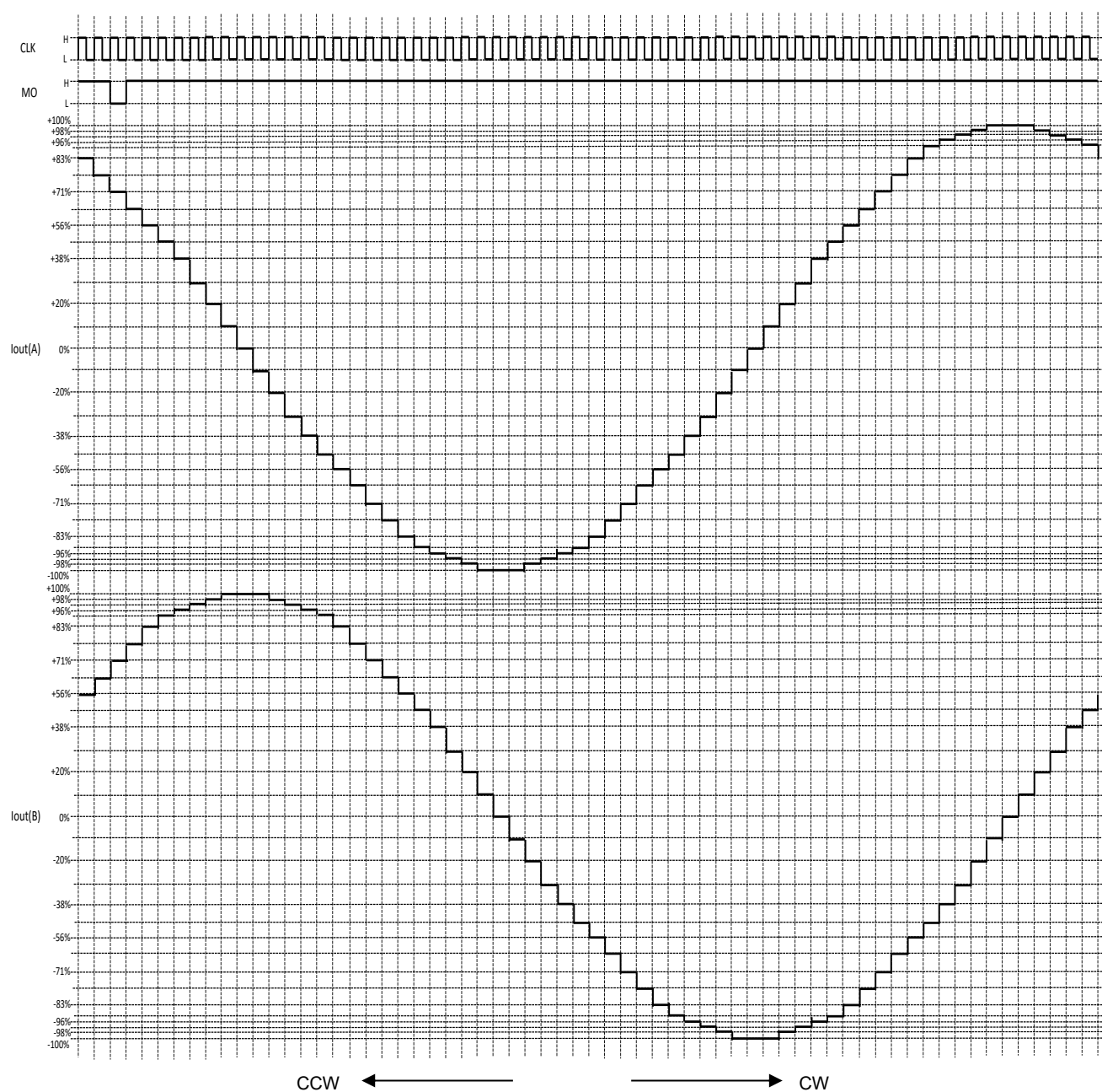
Figure 6.6 1/16 step resolution
