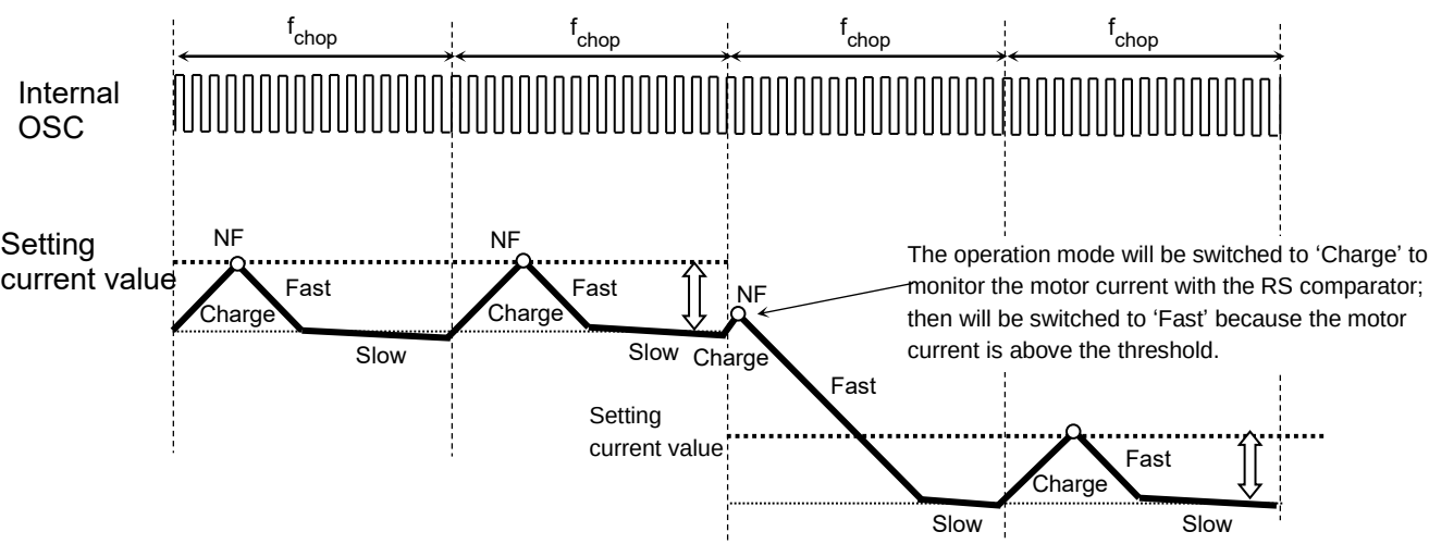
Figure 6.13 When the next current step is lower
