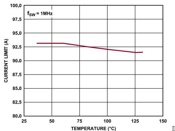
Figure 18. Current Limit vs. Temperature
