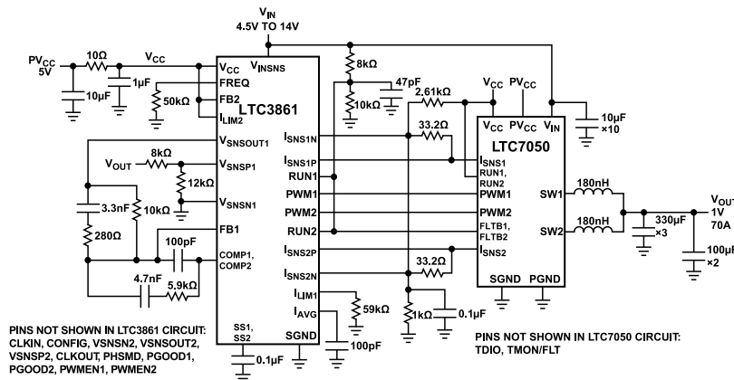
Figure 1. 12 V IN , 1 V/70 A OUT 1 MHz Dual-Phase POL Converter
