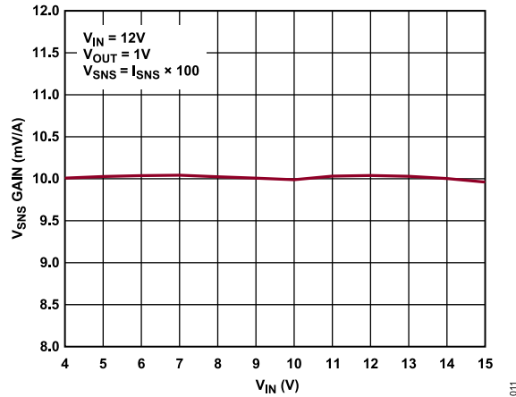
Figure 10. V_{SNS} Gain vs. V_{IN}
