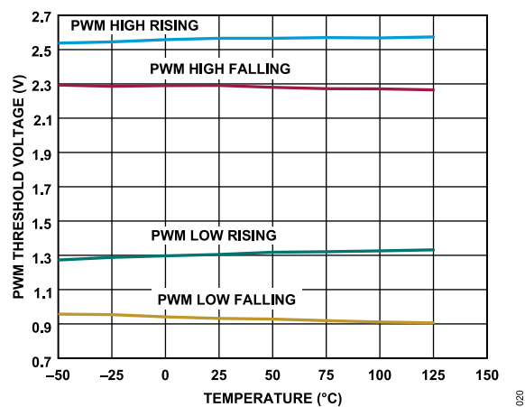
Figure 19. PWM Threshold vs. Temperature
