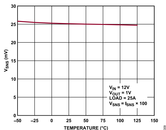
Figure 8. V_{SNS} vs. Temperature
