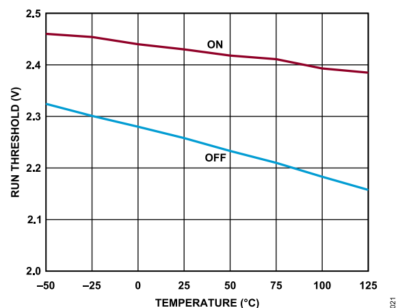
Figure 20. RUN Threshold vs. Temperature
