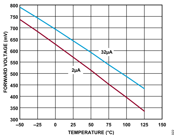
Figure 21. TDIO Forward Voltage
