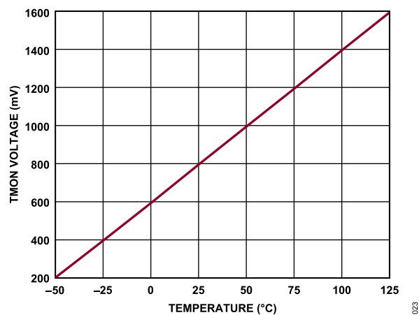
Figure 22. TMON vs. Temperature
