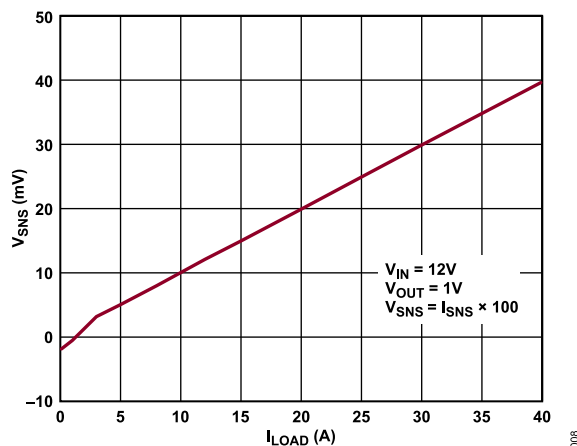
Figure 7. V_{SNS} vs. I_{LOAD}
