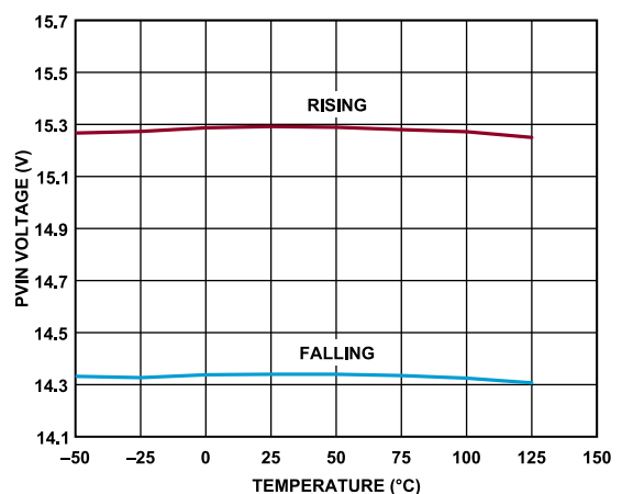
Figure 17. PV_{IN} OVLO vs. Temperature
