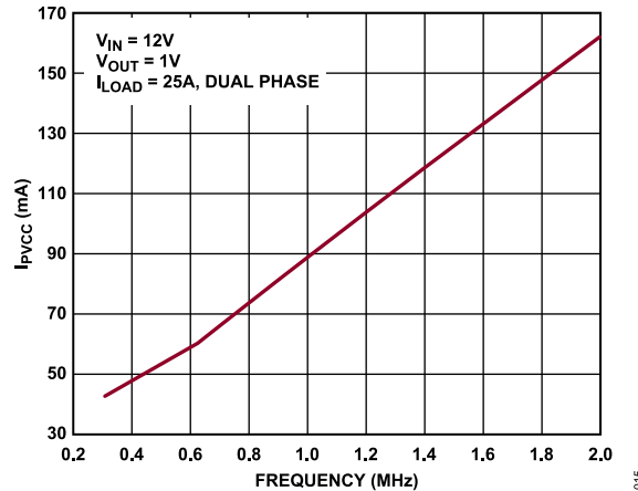
Figure 14. I_{PVCC} vs. Frequency
