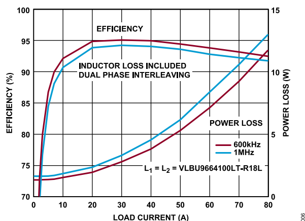
Figure 5. 12 V_{IN} to 1.8 V_{OUT} Efficiency
