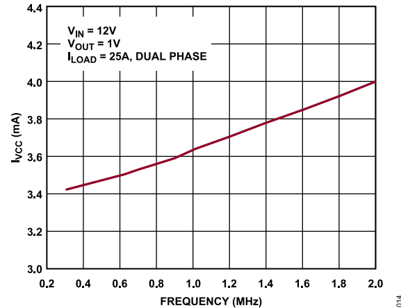
Figure 13. I_{VCC} vs. Frequency
