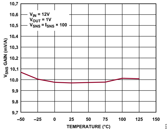
Figure 12. V_{SNS} Gain vs. Temperature
