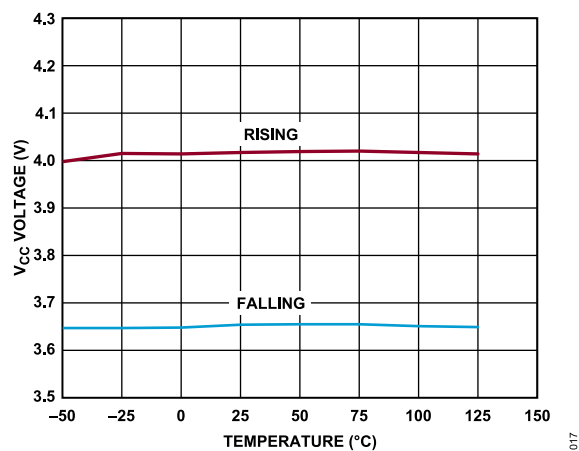
Figure 16. PV_{CC} UVLO vs. Temperature
