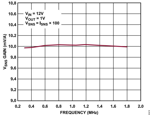
Figure 11. V_{SNS} Gain vs. Frequency
