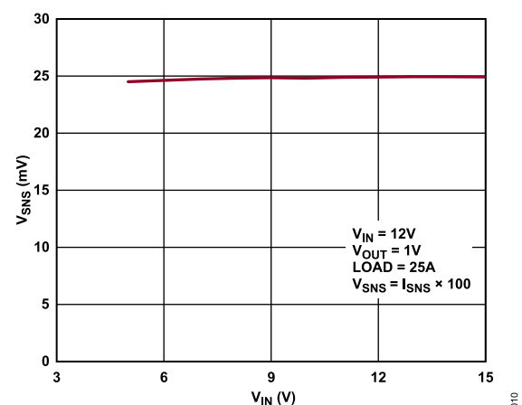
Figure 9. V_{SNS} vs. V_{IN}
