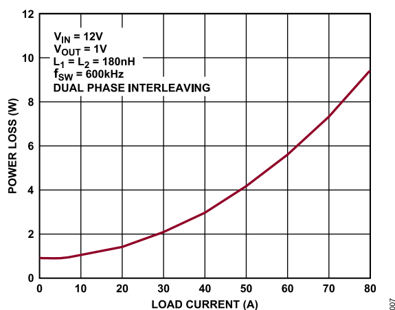
Figure 6. Power Dissipation vs. Load
