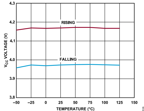
Figure 15. V_{CC} UVLO vs. Temperature
