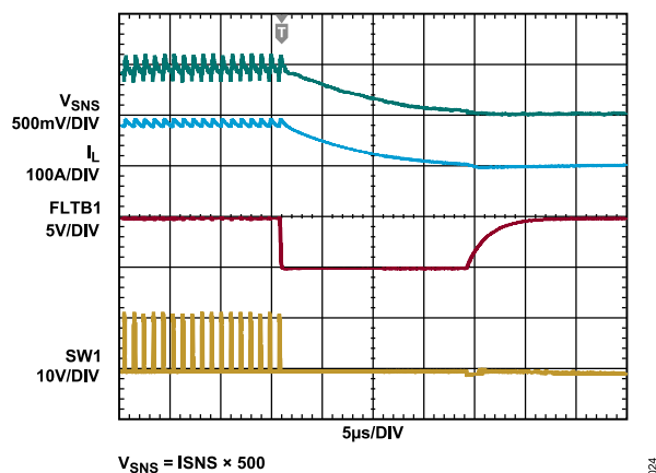
Figure 23. Overcurrent Protection
