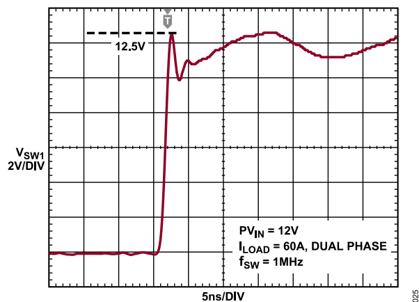
Figure 24. Switching Rising Edge
