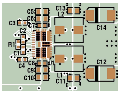
Figure 30. Example PCB Layout
