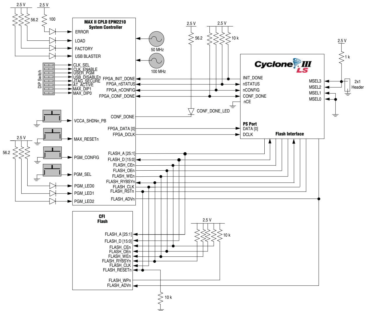
Figure 2-5. PFL Configuration
