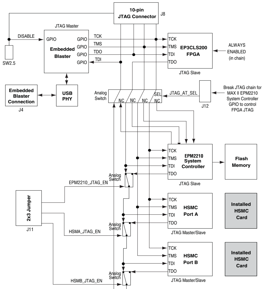
Figure 2-4. JTAG Chain
