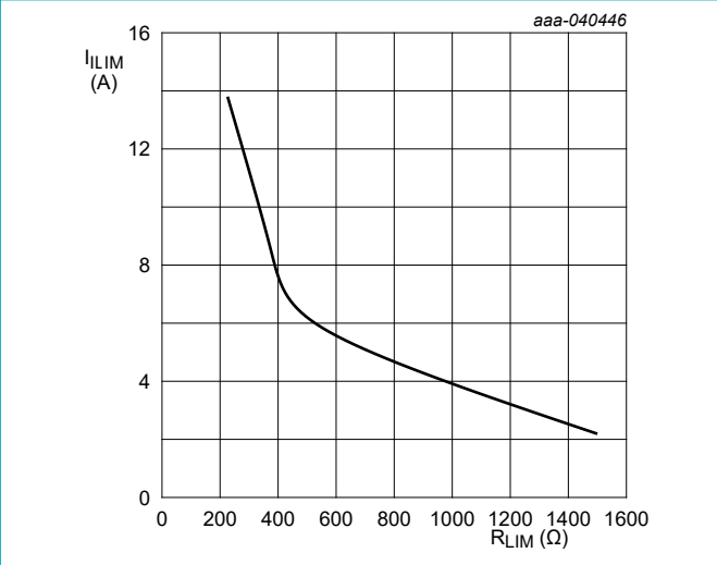
Fig. 12. Current limit ( I_{LIM} ) vs resistance ( R_{LIM} ) V_{IN} = 12 V; T_j = 25 \text{ }^\circ\text{C}
