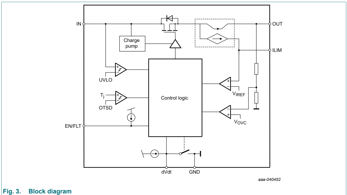
Fig. 2. Functional diagram
