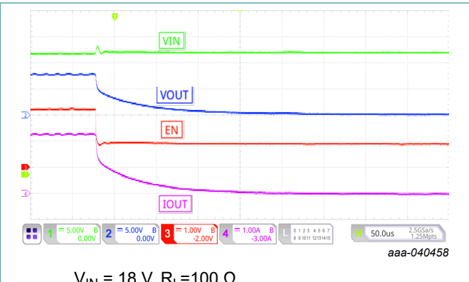
Fig. 19. Over temperature shutdown due to persistent input over voltage
