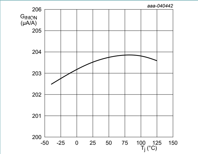
Fig. 8. Current gain ( G_{IMON} ) vs junction temperature V_{IN} = 12 V
