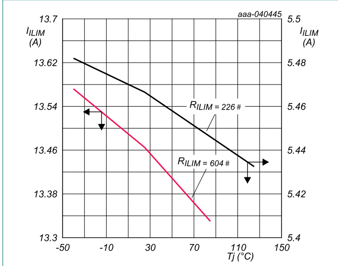
Fig. 11. Current limit ( I_{LIM} ) vs junction temperature V_{IN} = 12 V
