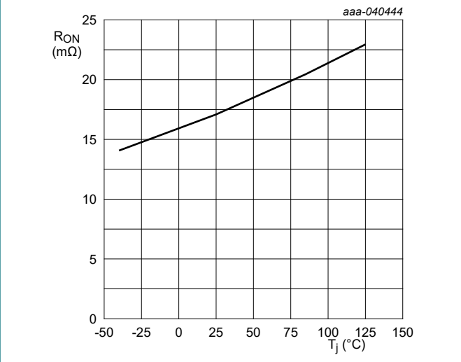
Fig. 10. On-state resistance ( R_{ON} ) vs junction temperature V_{IN} = 12 V
