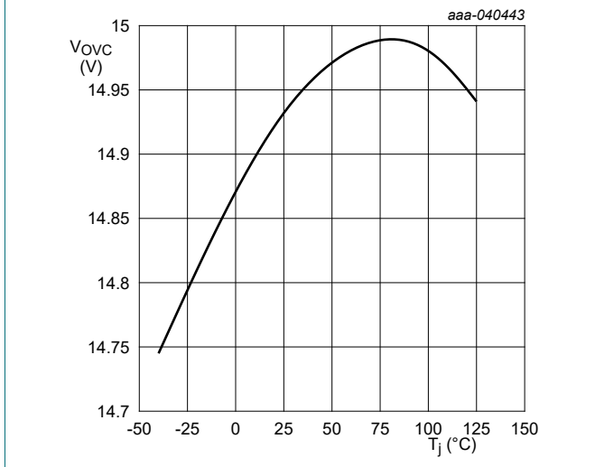
Fig. 9. Output clamp voltage ( V_{OVC} ) vs junction temperature V_{IN} = 18 V
