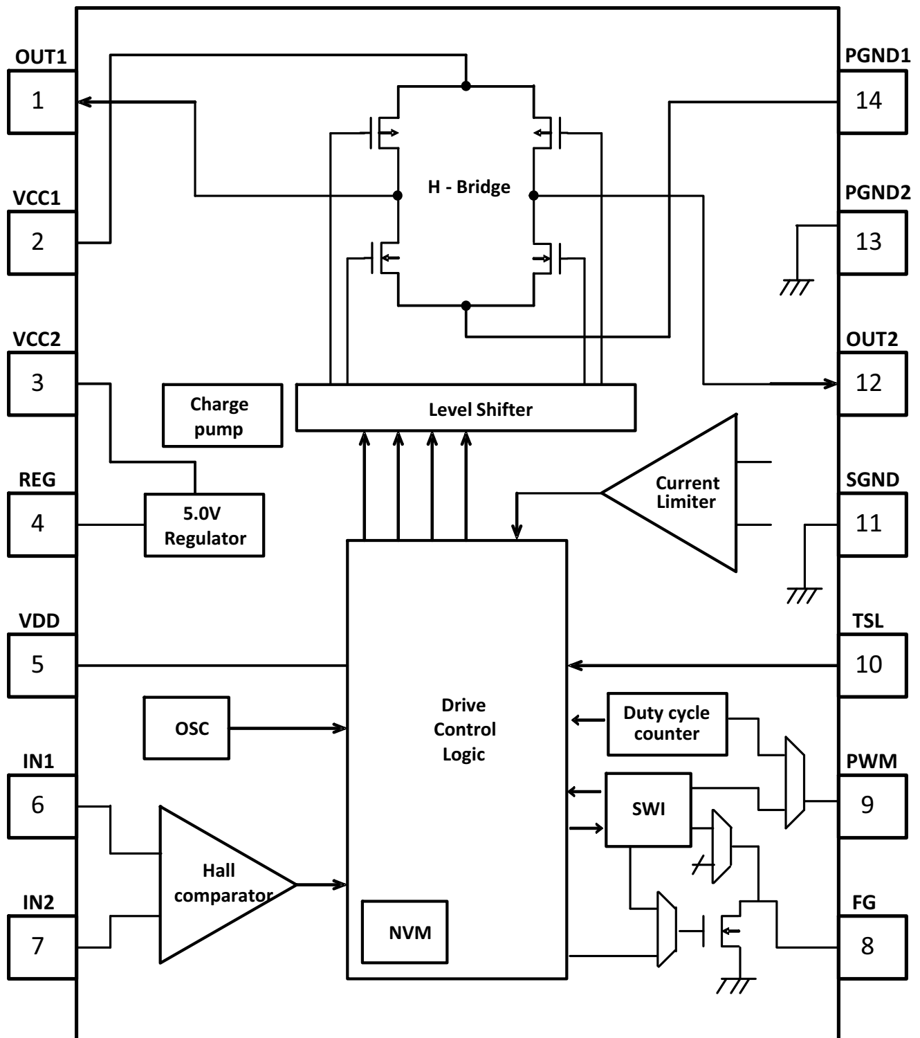
Figure 2. Block Diagram
