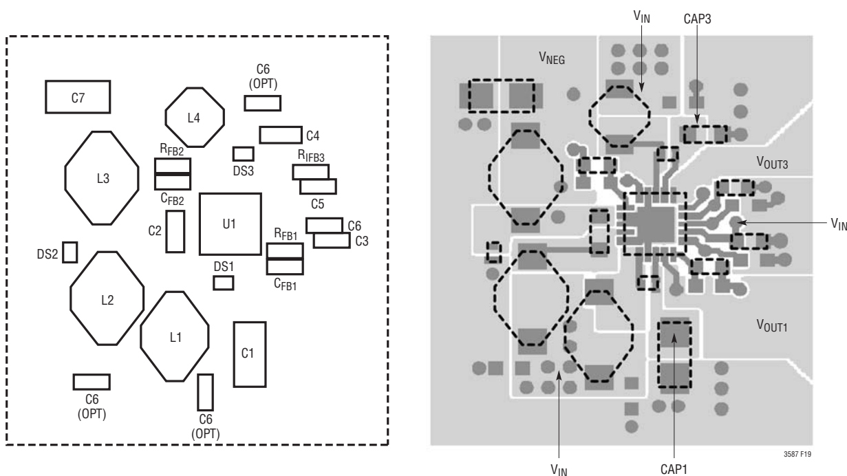
Figure 19. Recommended Component Placement
