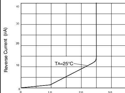
Reverse Characteristics
