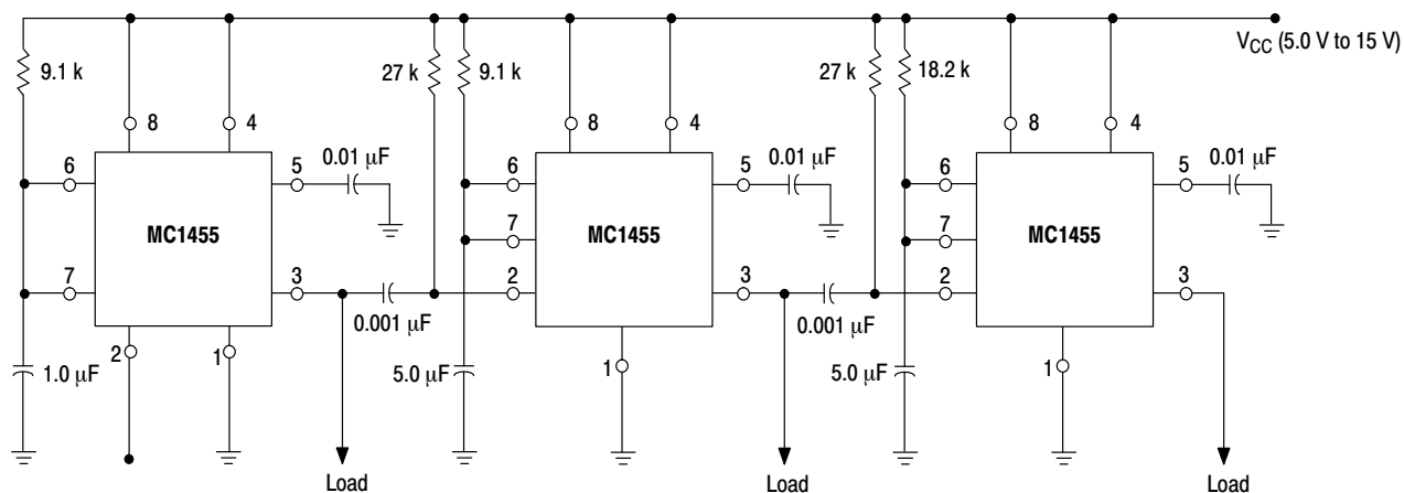
Figure 26. Sequential Timer
