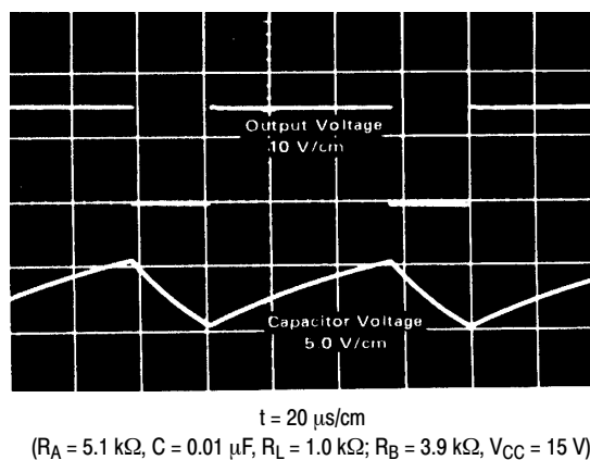
Figure 18. Astable Waveforms
