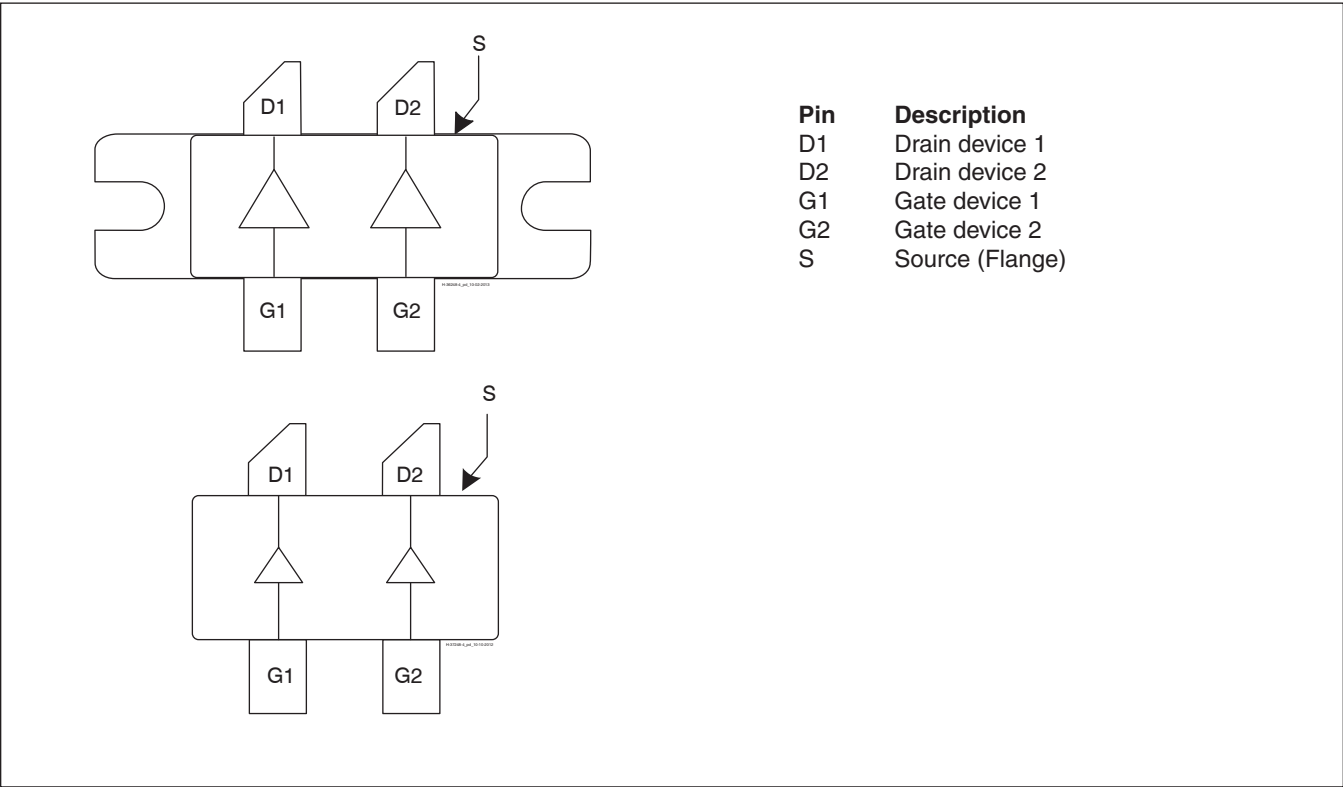
Lead connections for PTVA042502EC and PTVA042502FC
